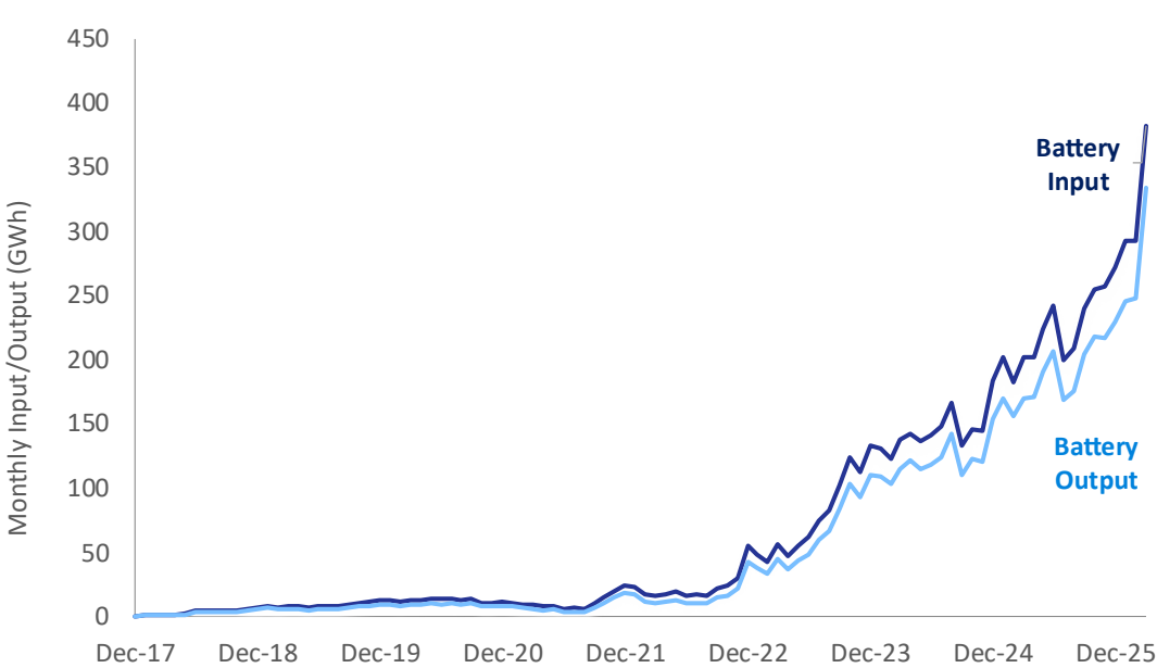
Chart 2: Monthly Great Britain (GB) grid-scale battery input and output (GWh), 2017 to March 2026
