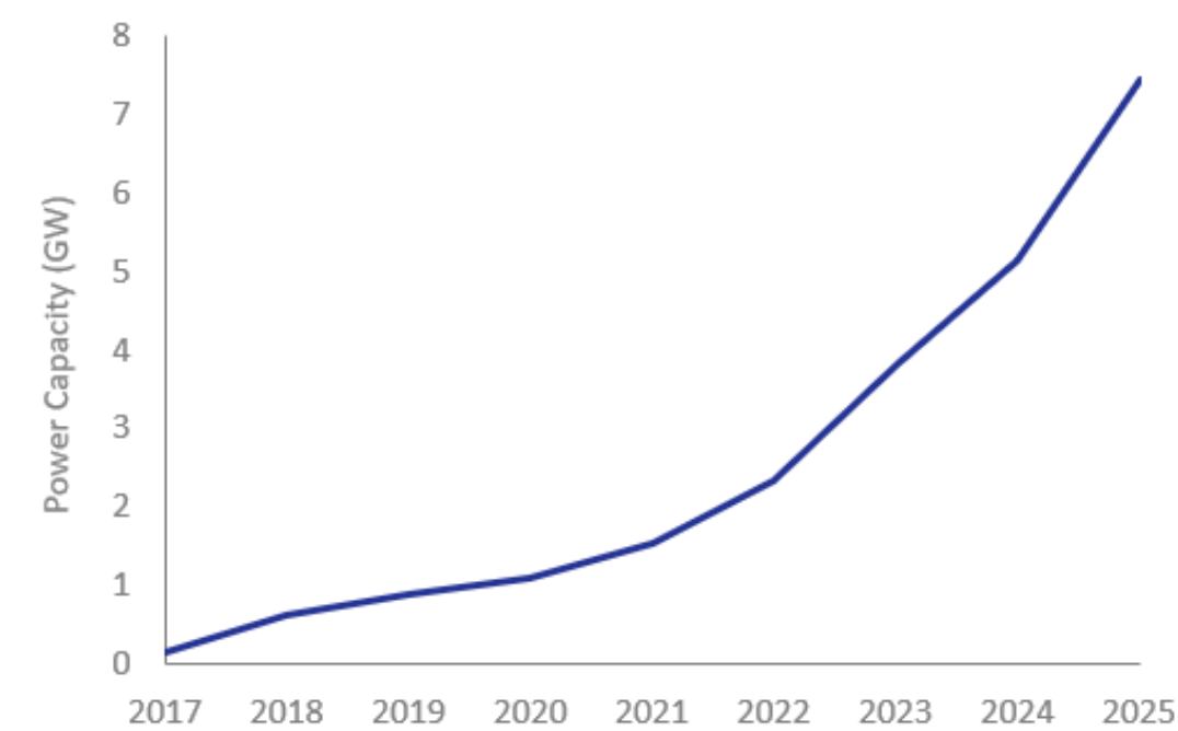
Chart 1: Annual UK grid-scale battery power capacity (GW), 2017 to 2025
