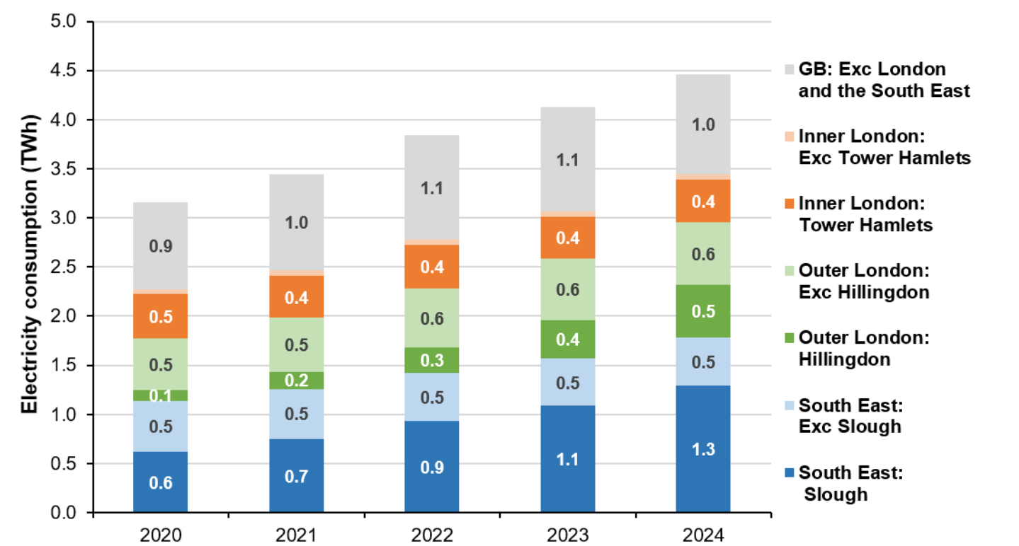
Chart 1: Data centre electricity consumption in Great Britain, 2020-2024
