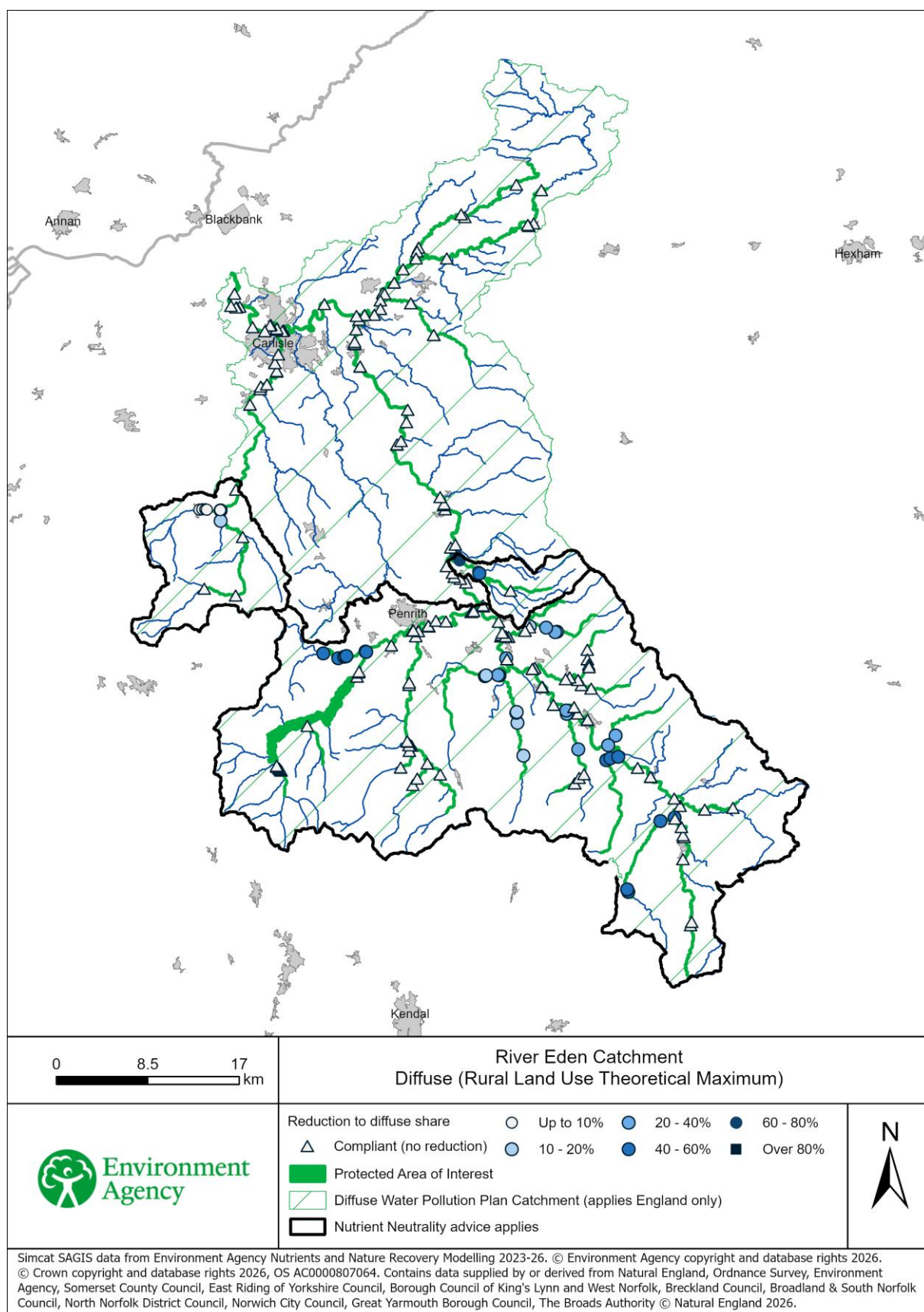
Map 9. Estimated reductions needed in diffuse phosphate concentrations to meet the diffuse share of the target in the 2030 Theoretical Maximum Scenario. Estimated diffuse reductions are improved marginally when compared to the 2030 Full Regulation scenario. The estimated reductions in parts of the southern catchment are mainly 10% to 60%, but with isolated locations where 60% to 80% reductions are needed.
