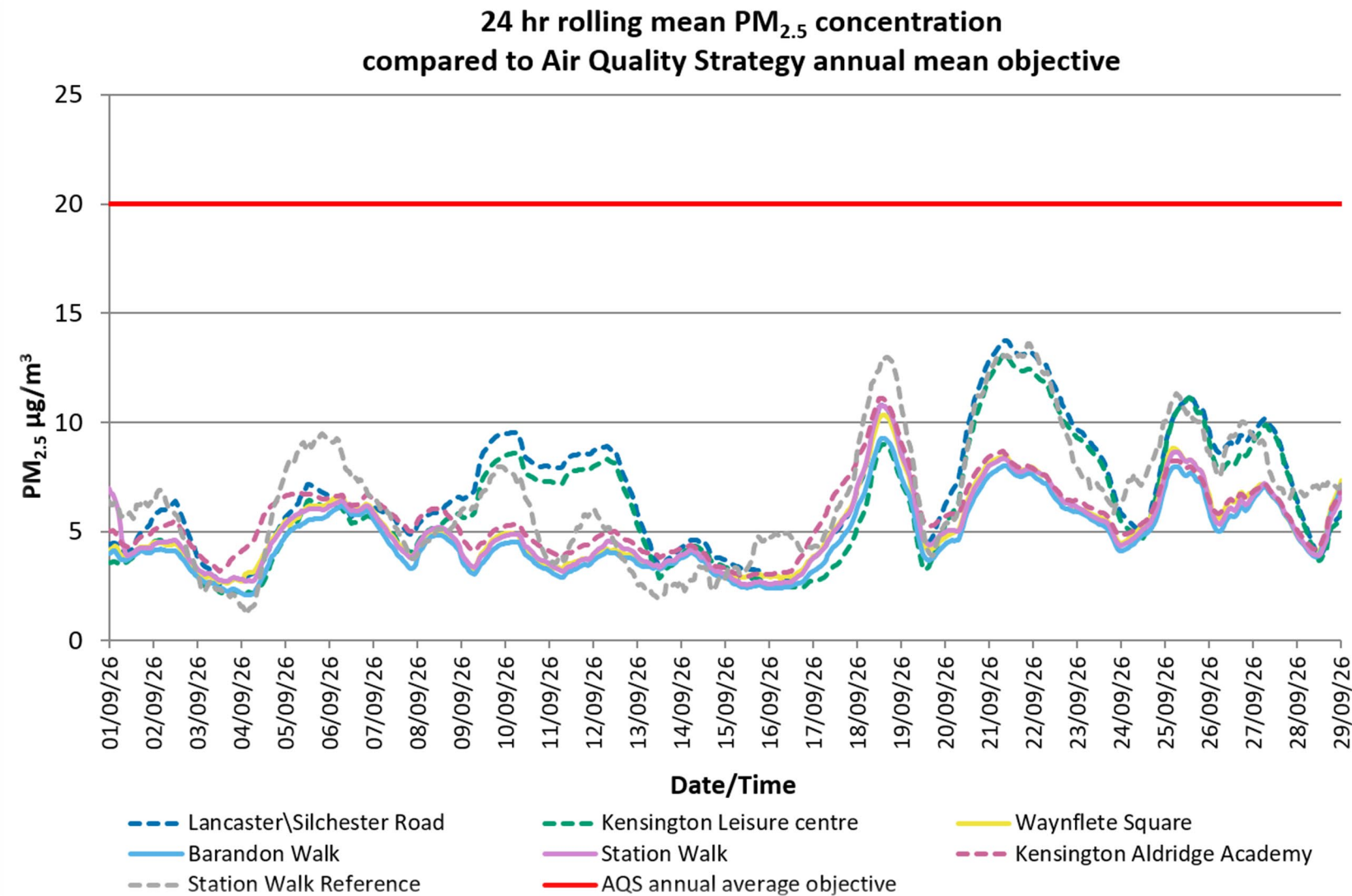
Figure 5. 24-hour rolling average particulate matter (PM 2.5 ) concentrations over the last 4 weeks for each of the 7 UKHSA - commissioned monitoring locations
