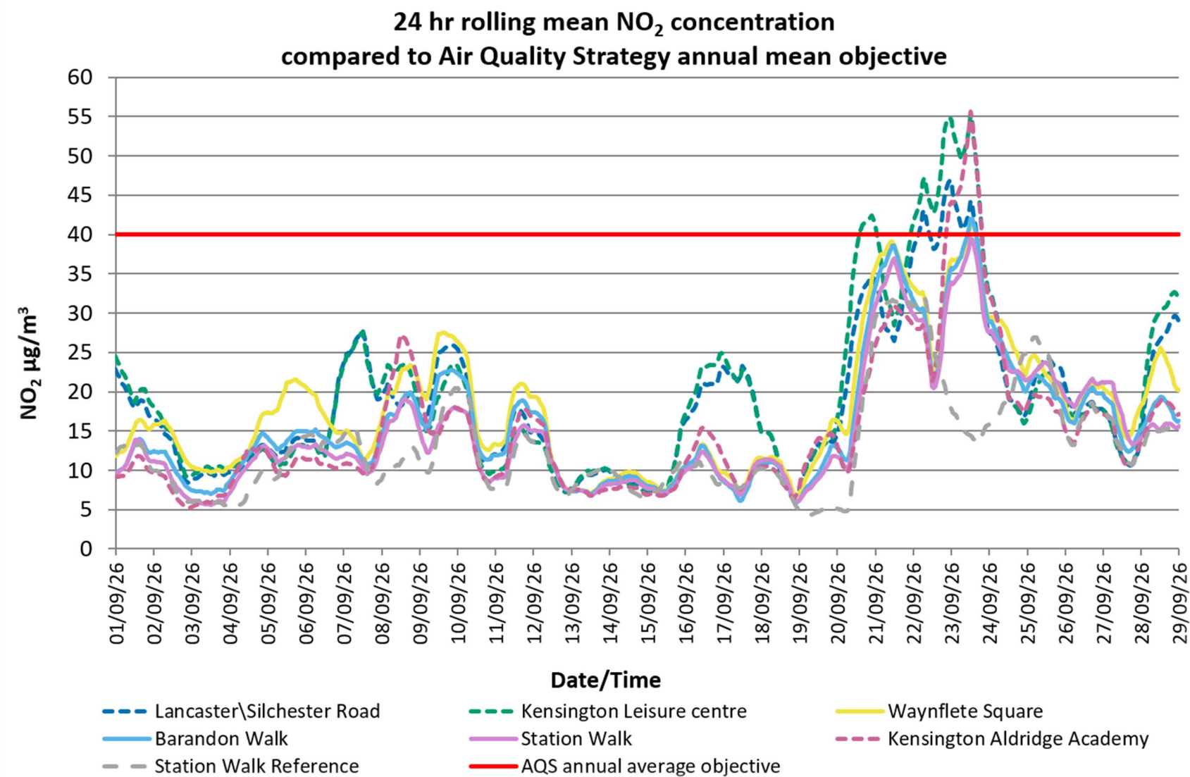
Figure 7. 24-hour rolling average nitrogen dioxide (NO 2 ) concentrations over the last 4 weeks for each of the 7 UKHSA-commissioned monitoring locations
