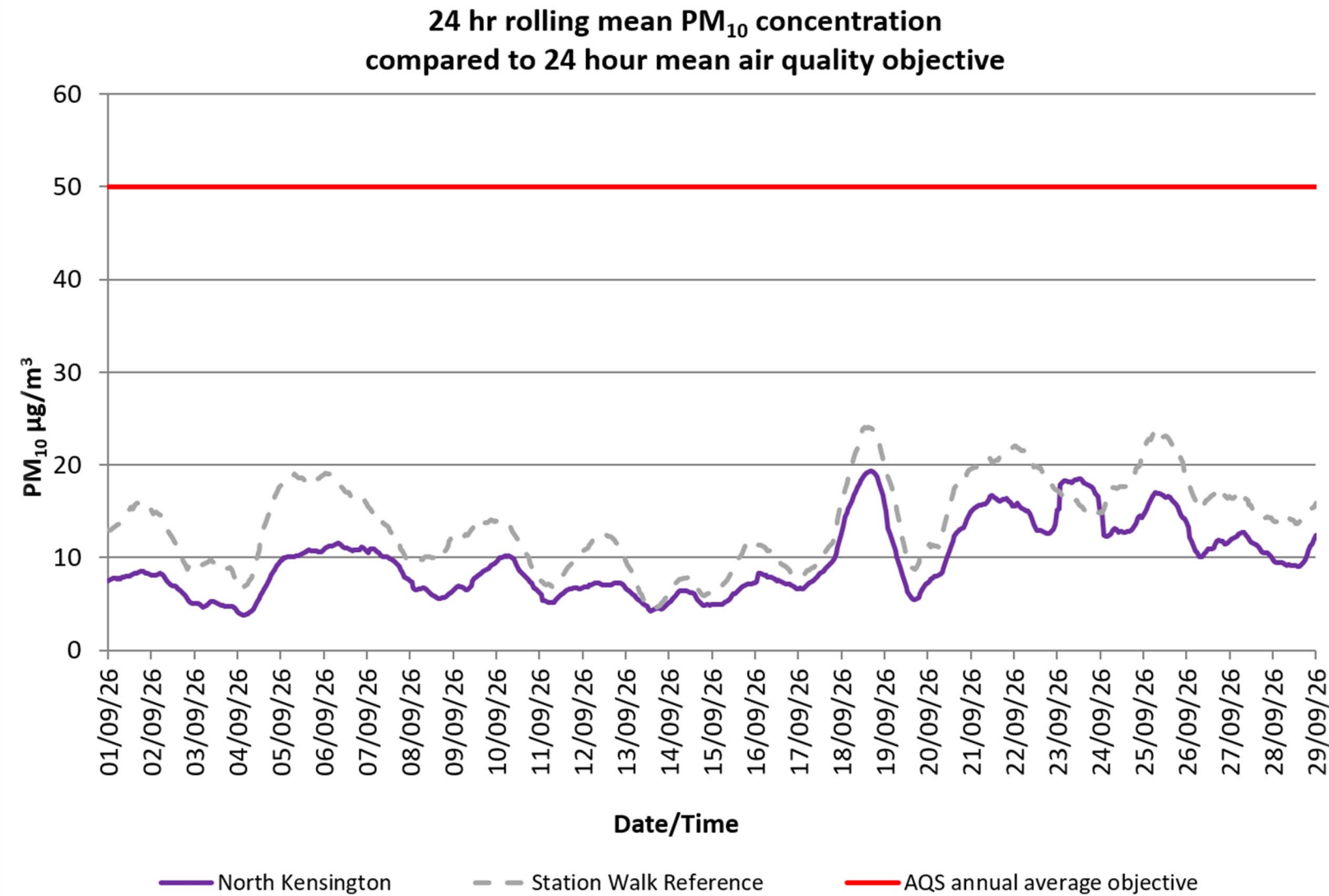
Figure 3. 24-hour rolling average particulate matter (PM 10 ) concentrations over the last 4 weeks at the UKHSA-commissioned monitoring reference site and the North Kensington London Air Quality Network site
