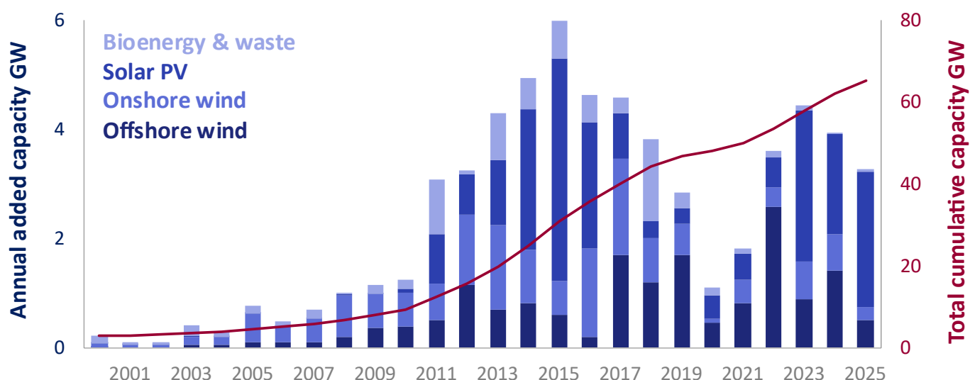
Chart 6.6 Annual added capacity 2000 to 2025 (DUKES Table 6.2)
