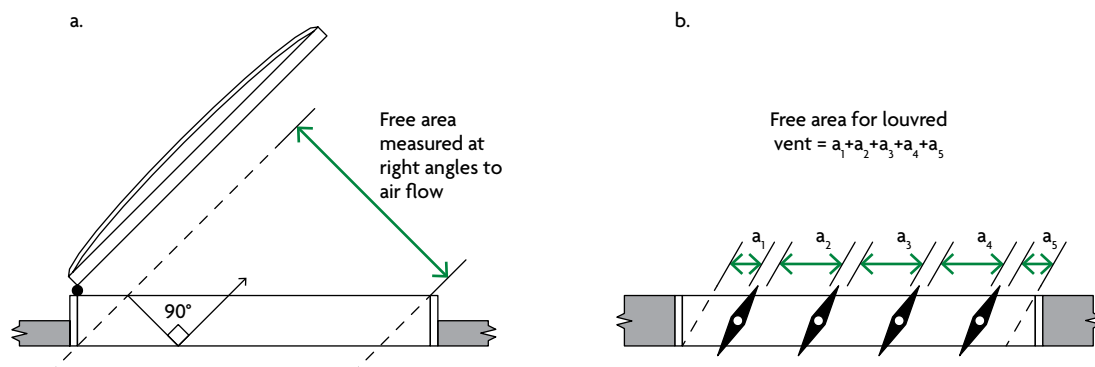
Diagram D7 Free area of smoke ventilators
