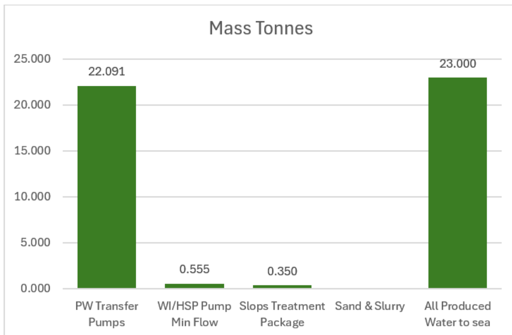
Figure 6 – Tonnes of oil in produced water discharged to sea by route during 2025.
