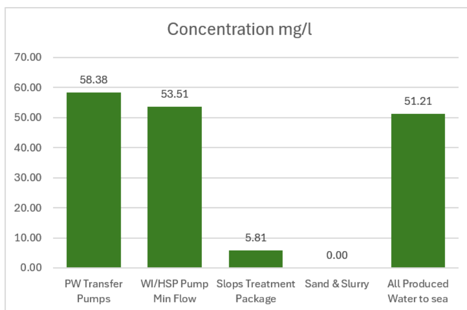
Figure 4 – Average Oil Concentration (mg/L) Of Produced Water by Route During 2025.
