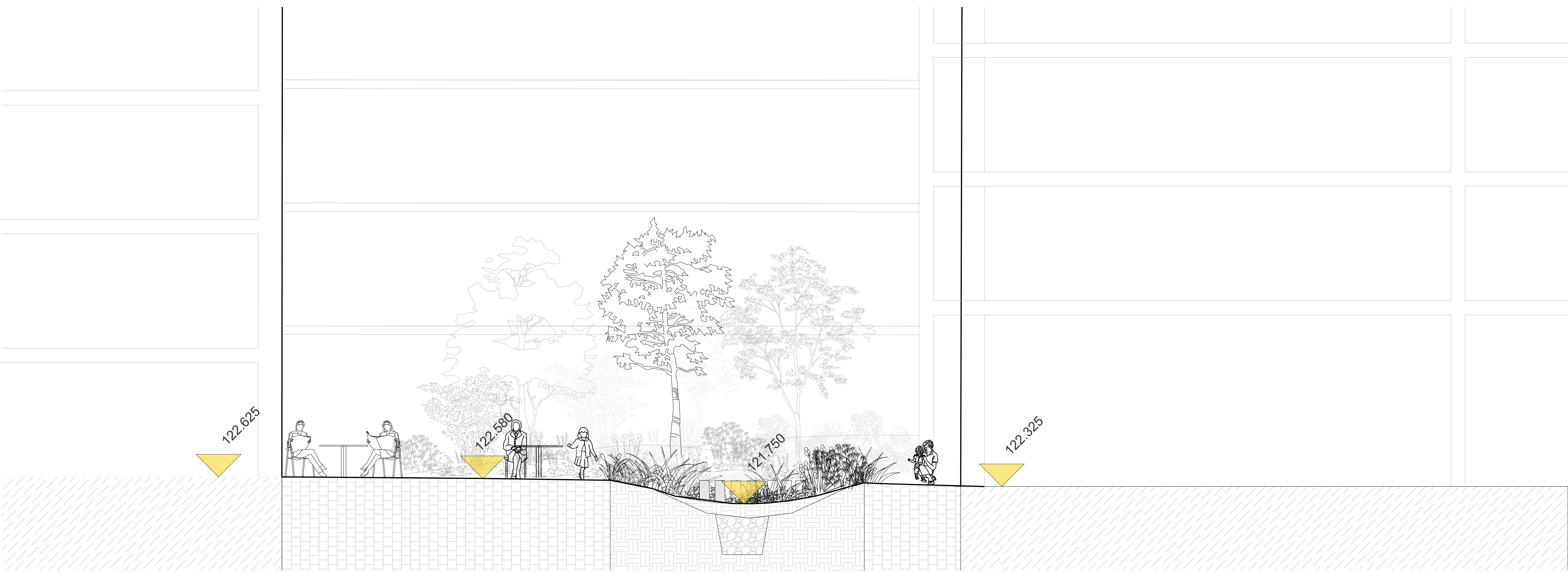
01 Section south bioswale AA Scale 1:50 @A1
