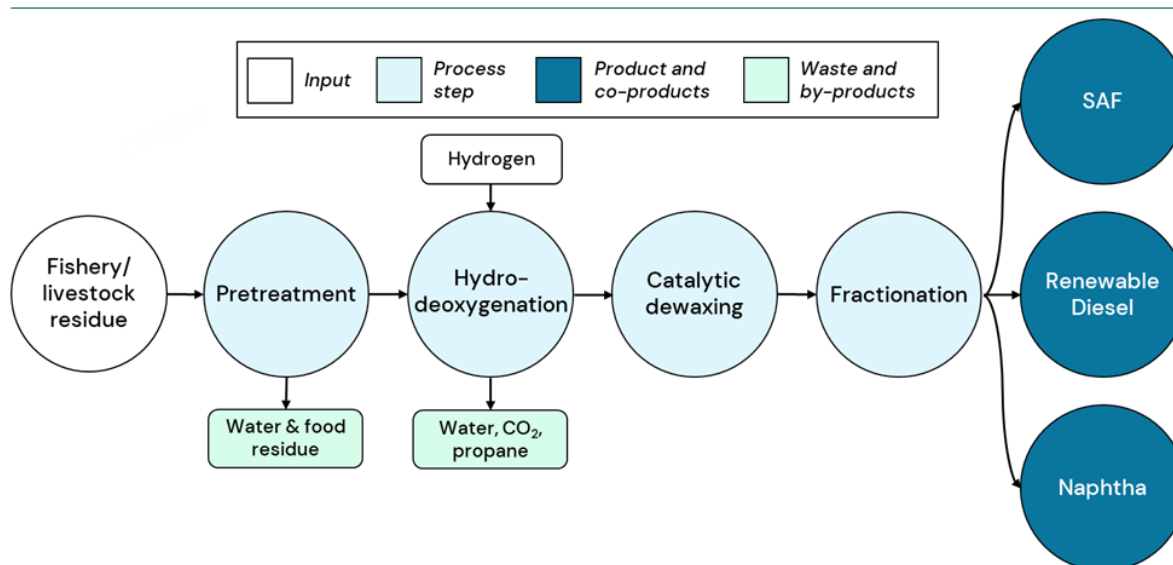
Figure 13 Process for HEFA SAF production
