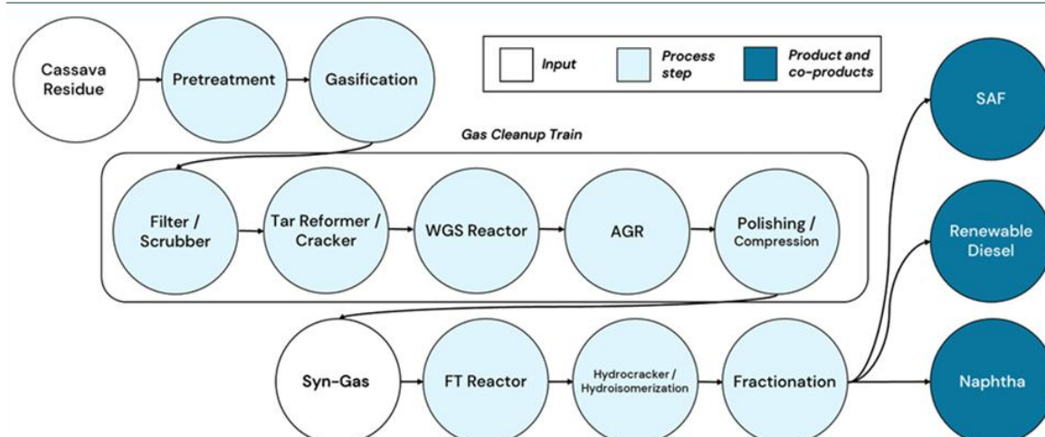
Figure 20 FT process flow
