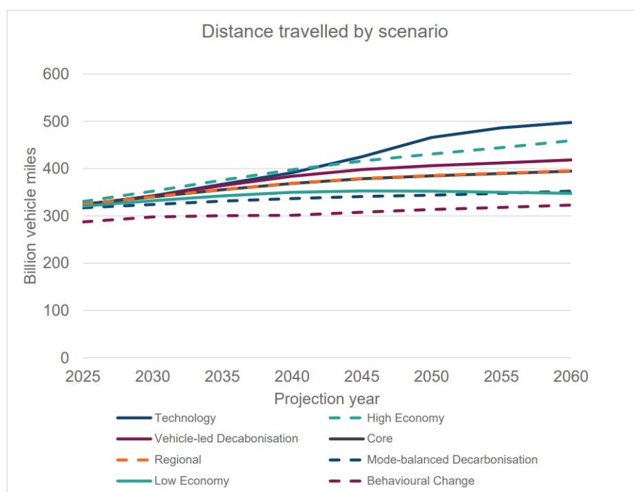
Figure 9 National Road Traffic Projections 2022, vehicle miles projections for England and Wales [note 667]
