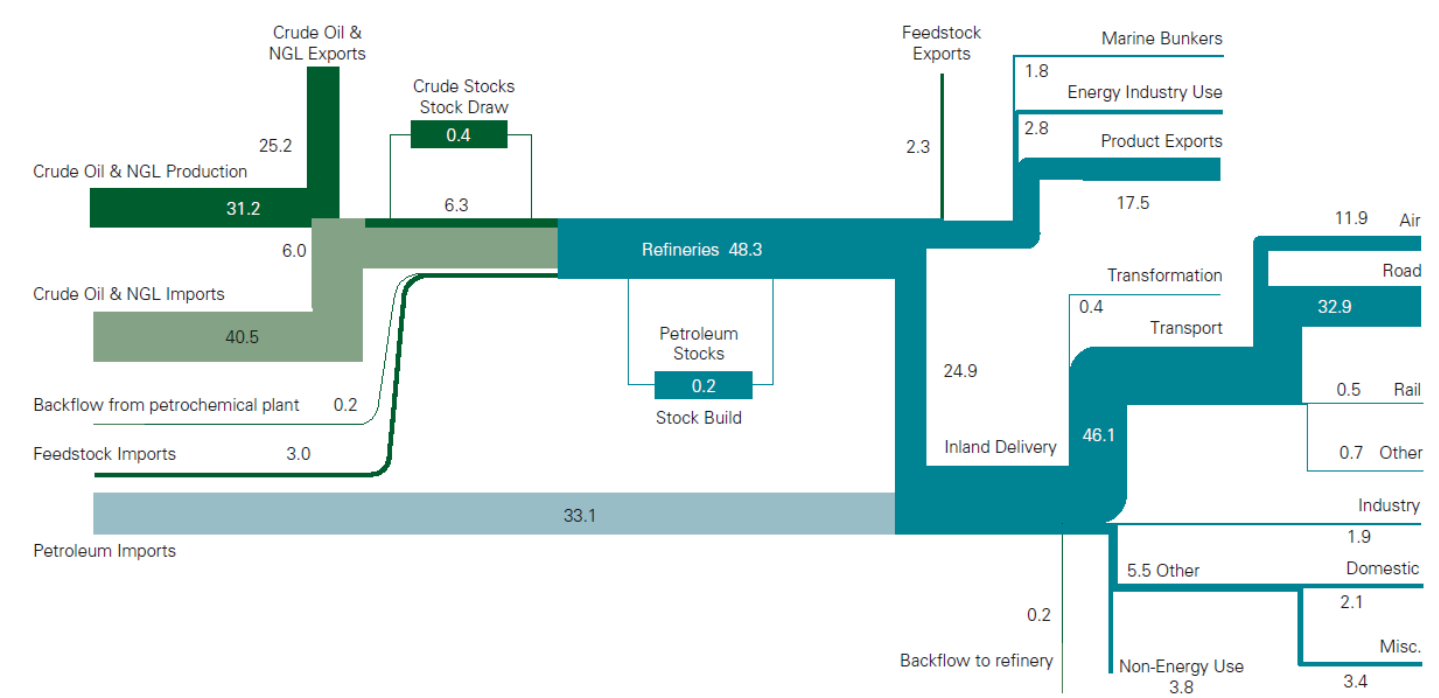
Chart H.2: Petroleum flow chart 2025 (million tonnes)
