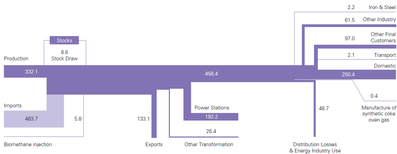
Chart H.3: Natural gas flow chart 2025 (TWh)
