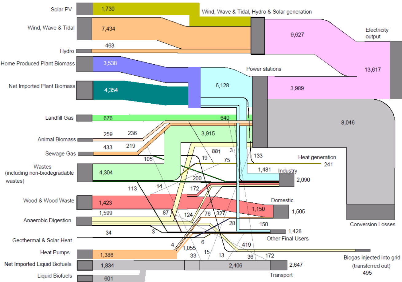
Chart H.5: Renewables flow chart 2025 (thousand tonnes of oil equivalent)
