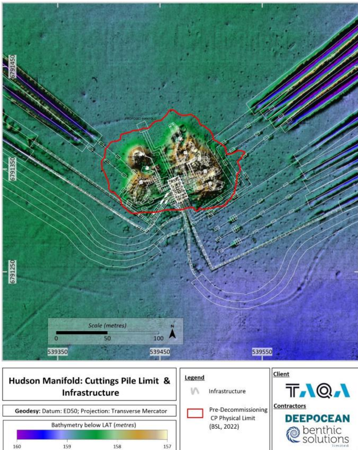
Figure 4-4 The Hudson Manifold Cuttings Pile(s)
