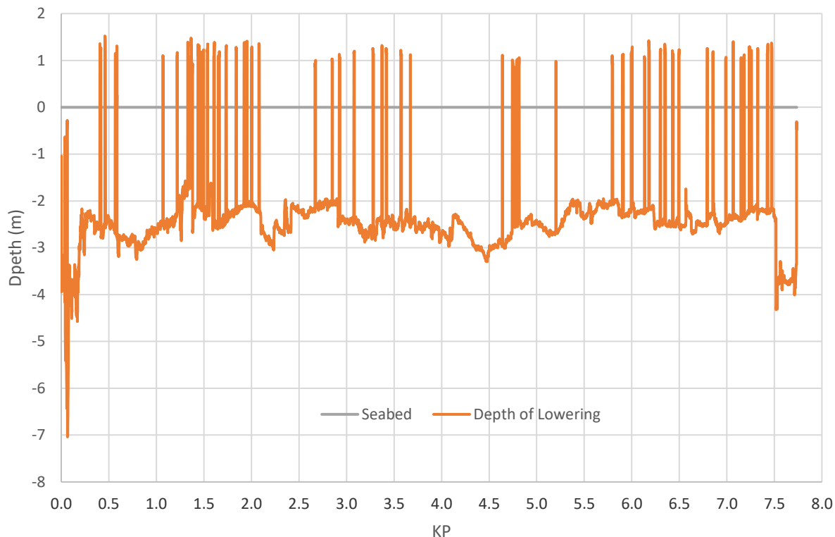
PL1852 Depth of Lowering
