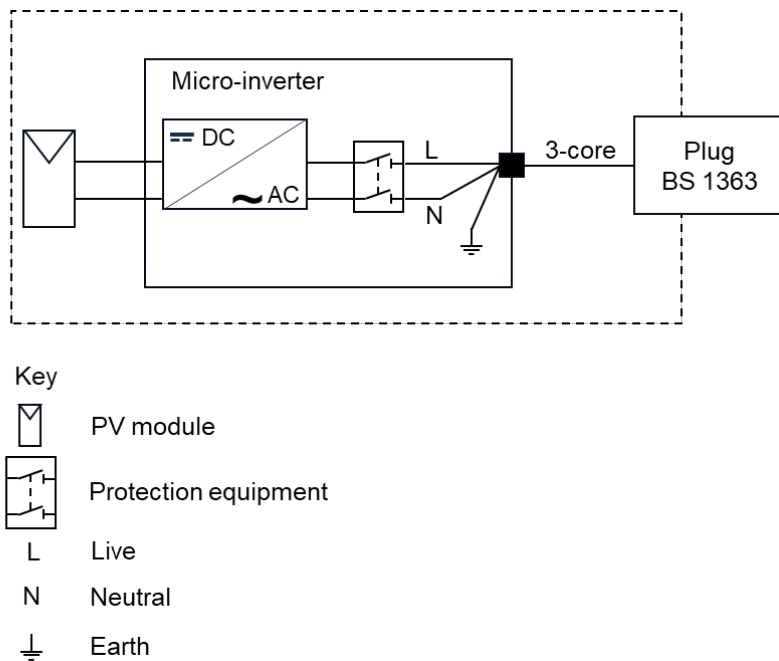
Figure 4- 1. Diagram of one-component plug-in solar device consisting of a single PV module with an integrated inverter. The DC-side connections are already established in the plug-in solar device..
