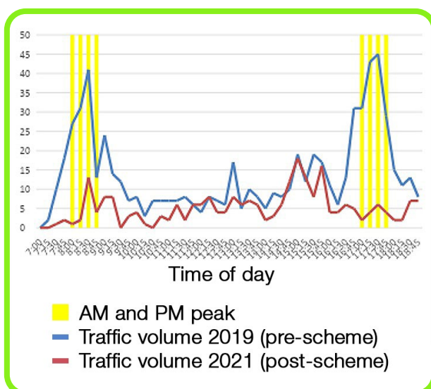
Figure 9: Total motor vehicle traffic along the length of Balls Farm Road west of Little John's Cross Hill.
