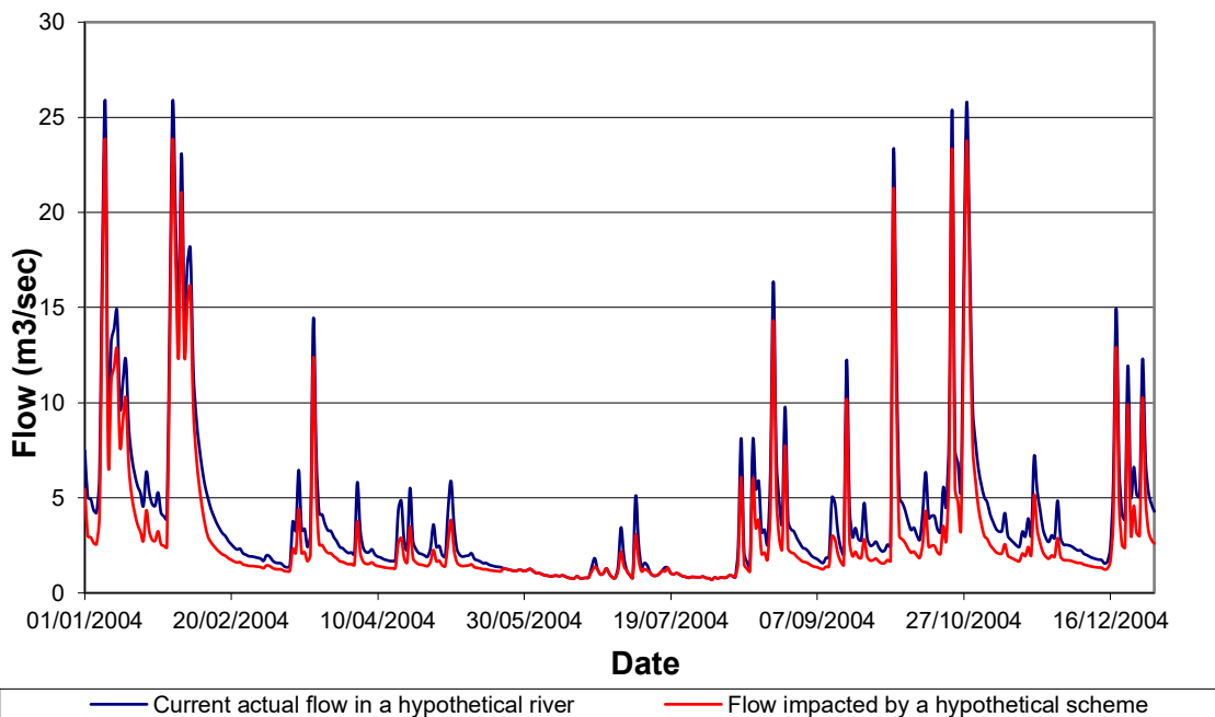
Figure 4.2: Hydrograph
