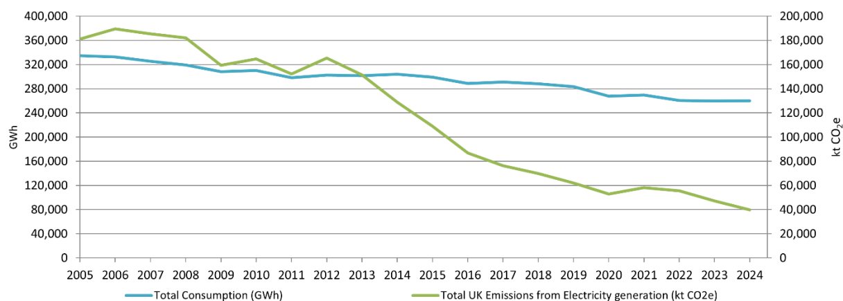
Figure 1 Time-series of electricity consumption and associated emissions in the UK
