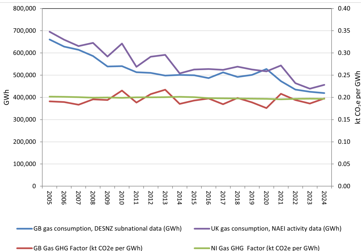
Figure 2 Natural gas consumption and emission factors, weather-corrected (Great Britain 2005-2014 and all of Northern Ireland) and not weather-corrected (Great Britain 2015-2024)
