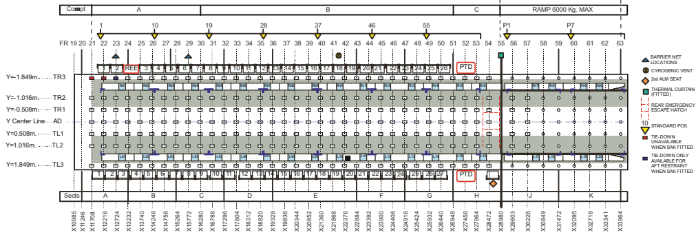
Toe Ramp Detail
