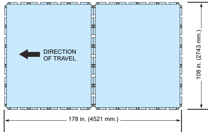
ADS - Double ACP - Dimensions of Usable Surface
