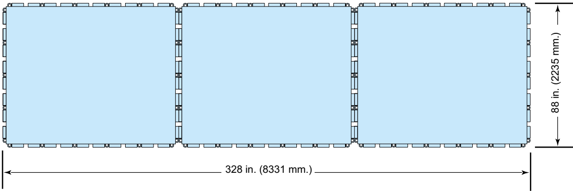
LOGS - Double ACP - Dimensions of Usable Surface
