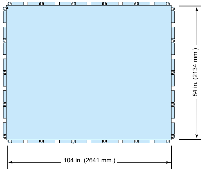
Useable Surface Area Of 463L ACP
