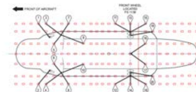
Image 3 - Chinook C17A tie-down scheme plan view
