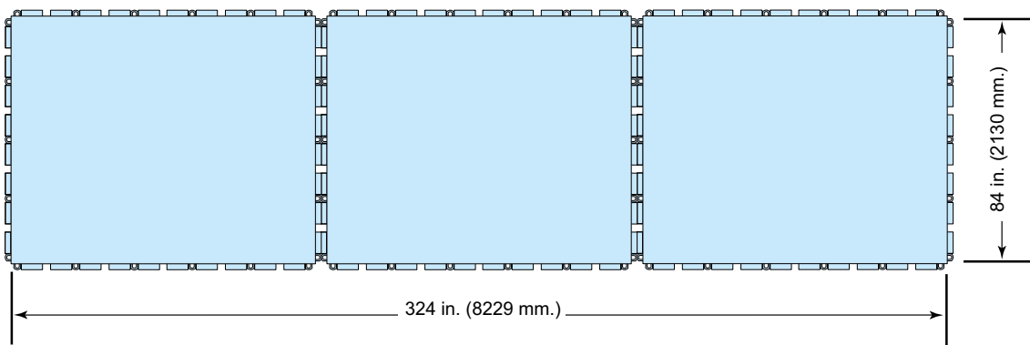
ADS - Triple ACP - Dimensions
