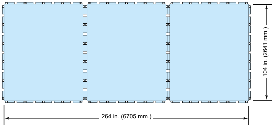
ADS - Triple ACP - Dimensions of Usable Surface
