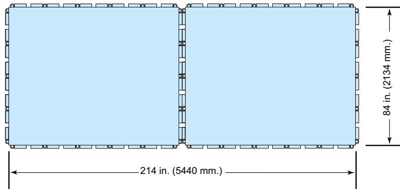
LOGS - Double ACP - Dimensions of Usable Surface
