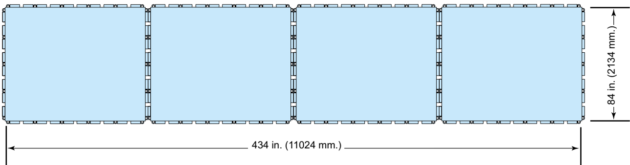
LOGS - Quad ACP - Dimensions of Usable Surface
