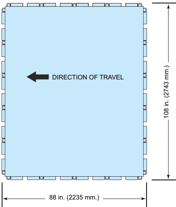
Overall Dimensions ADS
