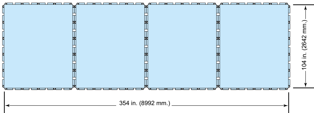
ADS - Quad ACP - Dimensions of Usable Surface
