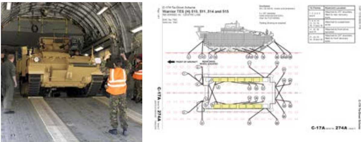
Image 1 - Warrior Armoured Tracked Vehicle on C-17A
