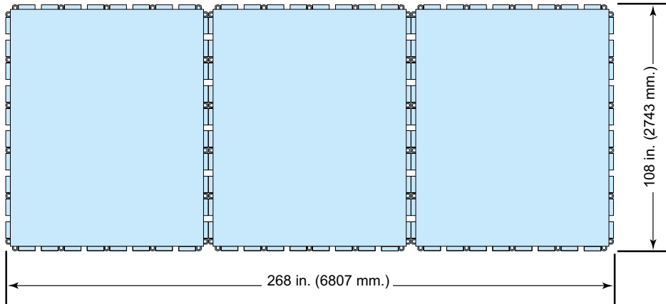
ADS - Triple ACP - Dimensions of Usable Surface
