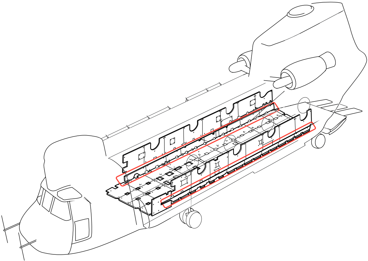
Areas that encroach on 90 in. Cargo Envelope -Buffer Board Panels LH and RH
