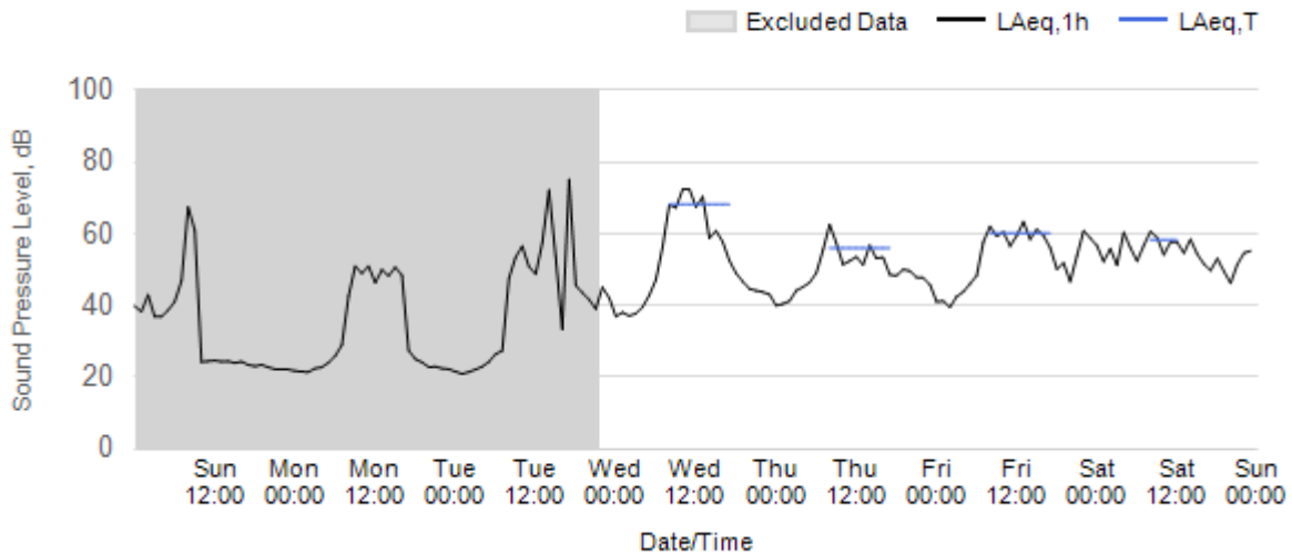
Worksite: A421 North Monitoring Ref: A421-N1 08 February 2026 to 14 February 2026
