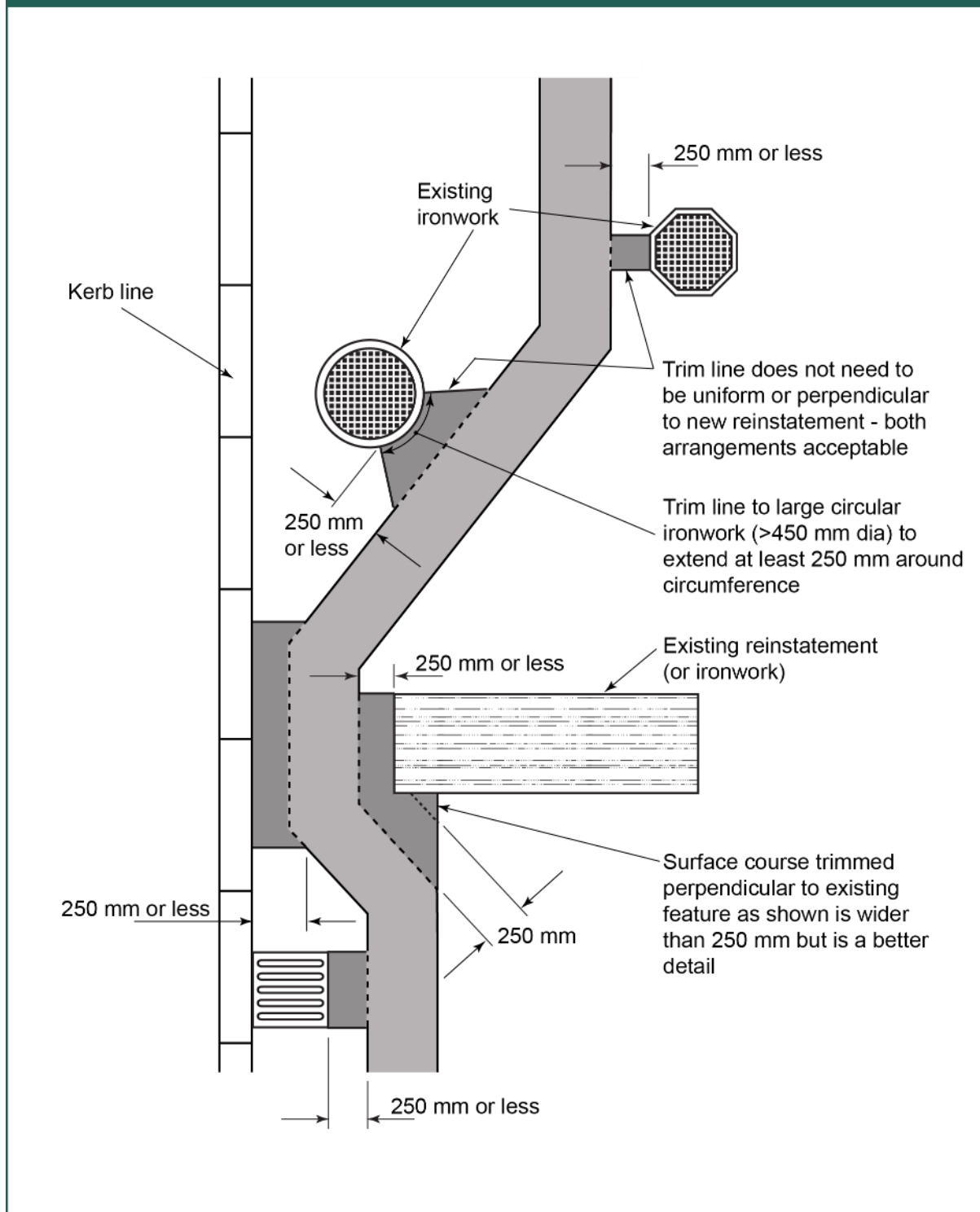
Figure S6.4 Edge requirements and trim lines in carriageways
