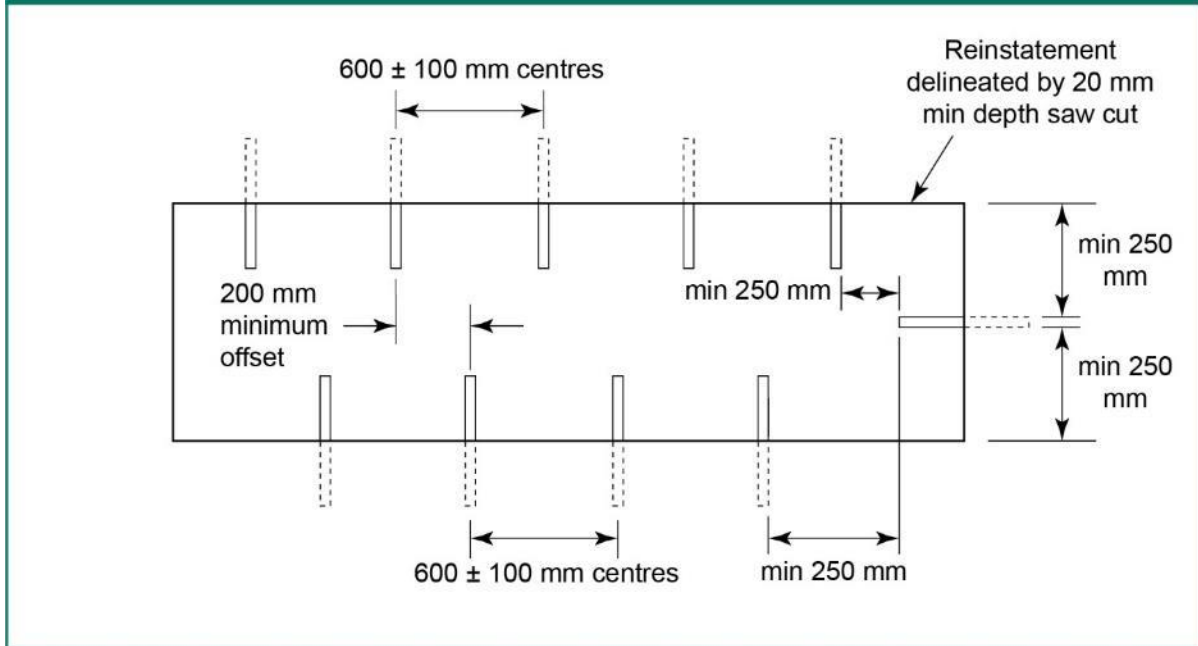
Figure S7.3 Dowel bar arrangement - plan view
