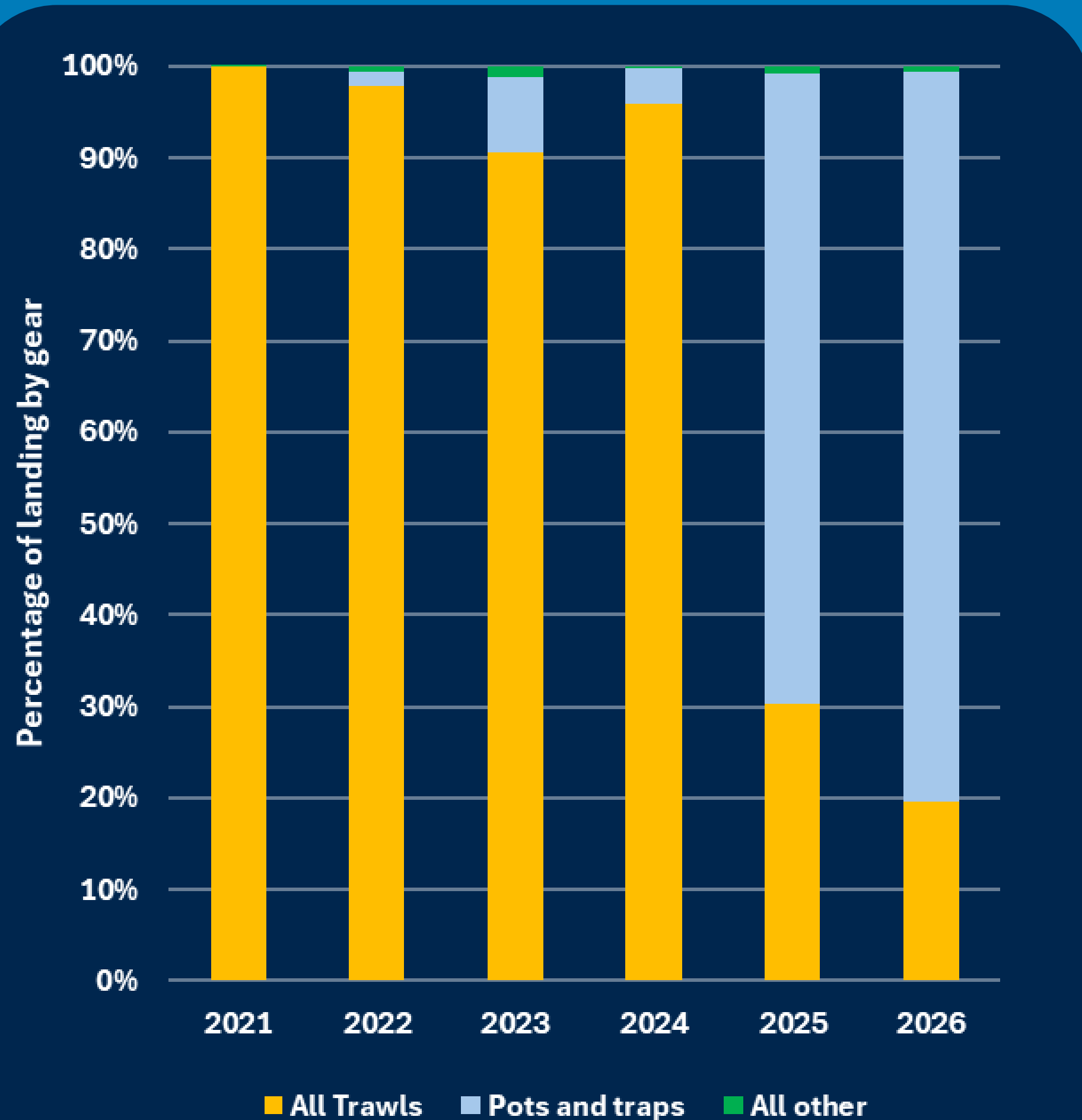
Figure 4. Percentage (%) of octopus landings, by gear type, from all UK vessels landed in all ICES areas. Data from 1 January 2021 to 14 April 2026. 'All other' gear represents all dredges, all nets, hooks and lines, and unspecified gears.
