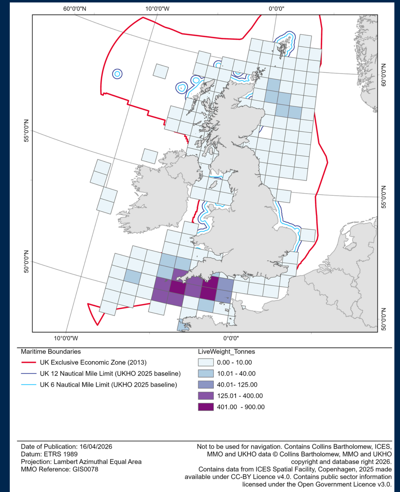
Figure 3. Heat map representing lives weight (tonnes) of octopus landed by UK vessels in each ICES rectangle. Data from the 1 January 2026 to 14 April 2026.
