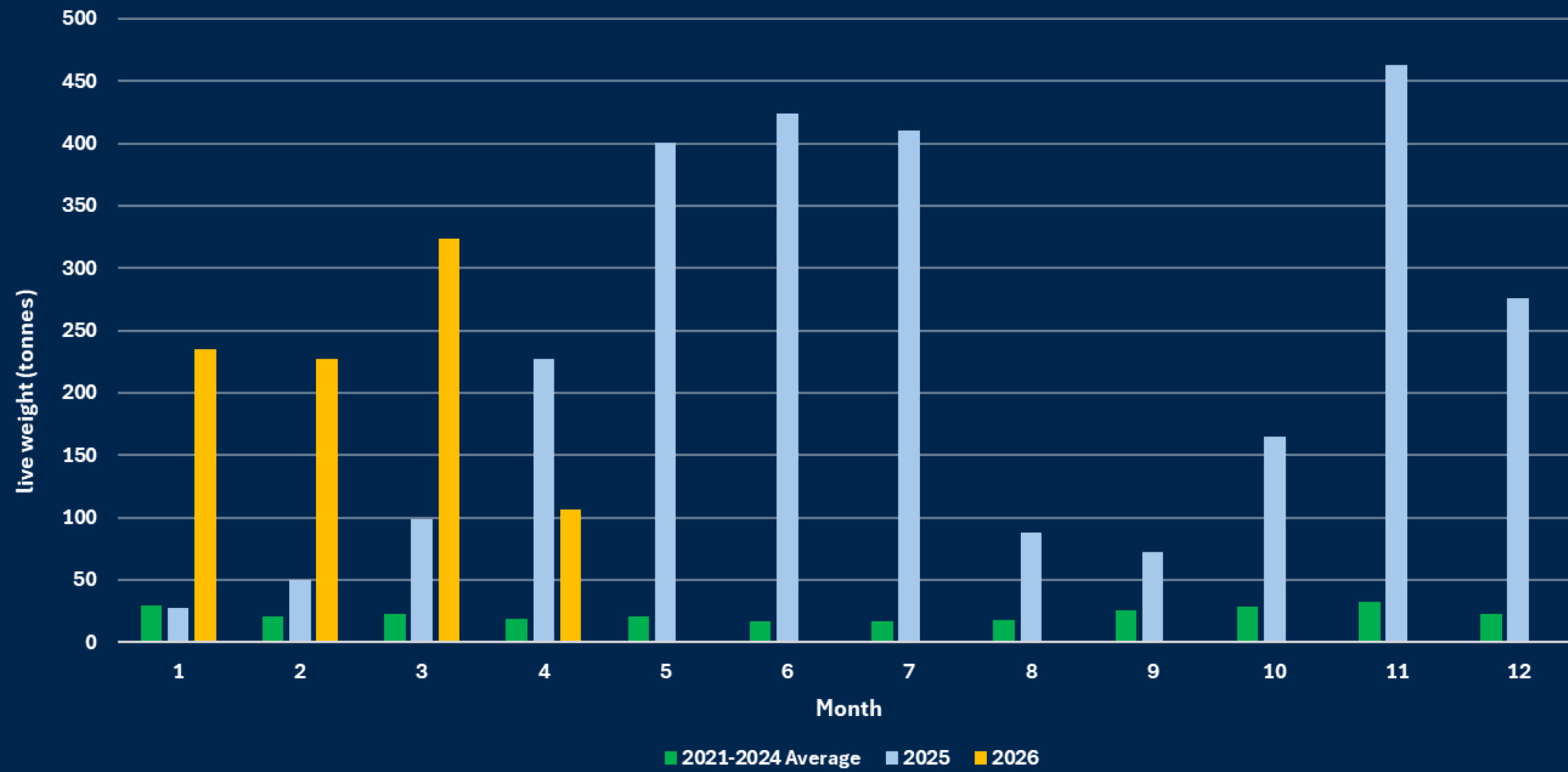
Figure 1. Monthly live weight (tonnes) of octopus landed from all UK vessels in all UK ports. (Months: January = 1, December = 12). Data from 1 January 2021 to 14 April 2026.
