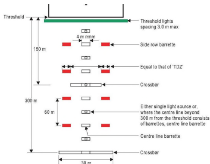
▶ Figure 3. Supplementary Approach Lighting ◀
