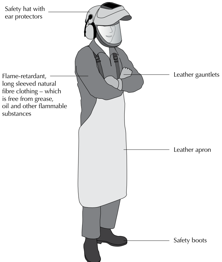
Figure 24.1 Examples of PPE for hot work
