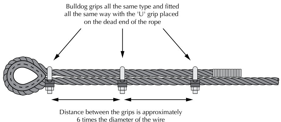
Figure 18.3 Use of bulldog grips
