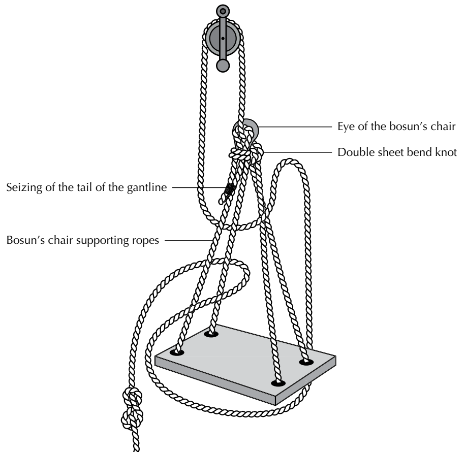
Figure 17.2 Bosun's chair
