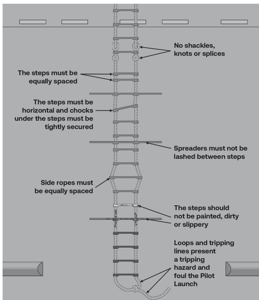
Figure 22.2 Checklist for safe means of access
