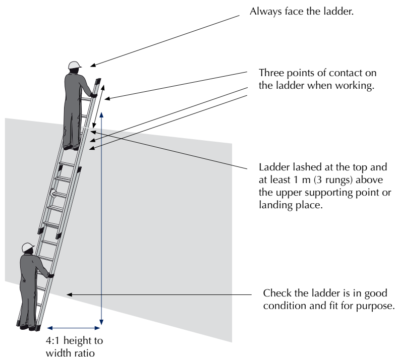
Figure 17.1 Portable ladder
