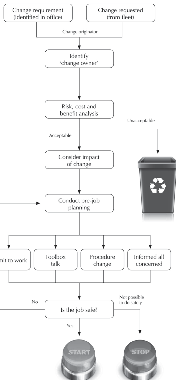
Figure 1.3 Procedures for simple and complex changes
