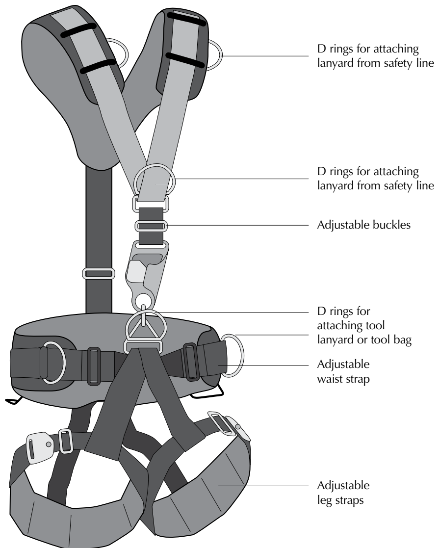
Figure 8.2 A five-point harness
