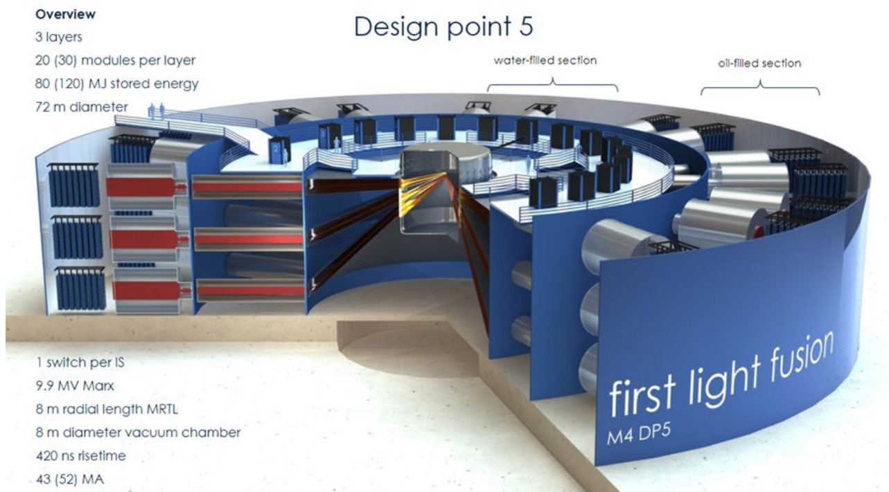
Figure 15 – Render of Machine 4
