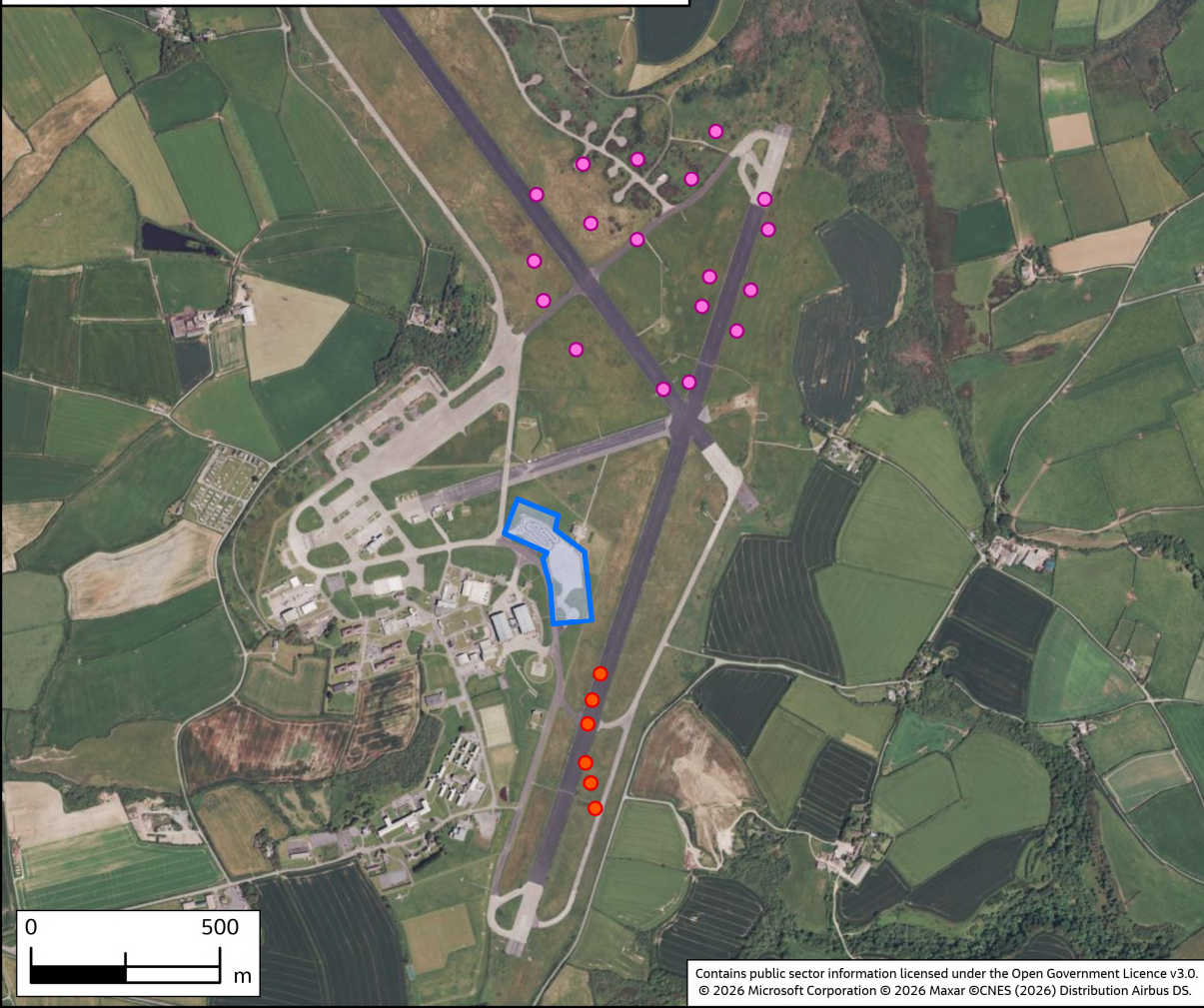
Layout 3 - Conceptual Layout Plan December 2024
