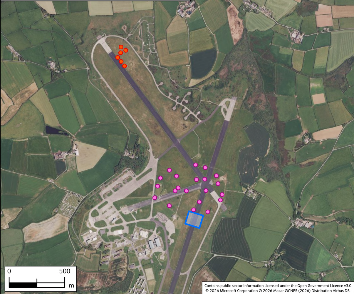
Layout 3 - Conceptual Layout Plan December 2024
