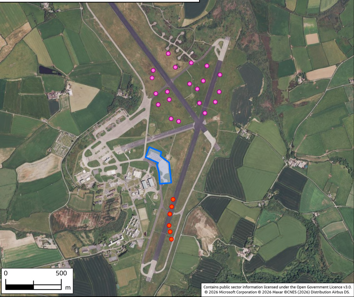
Layout 4 - Conceptual Layout Plan January 2025
