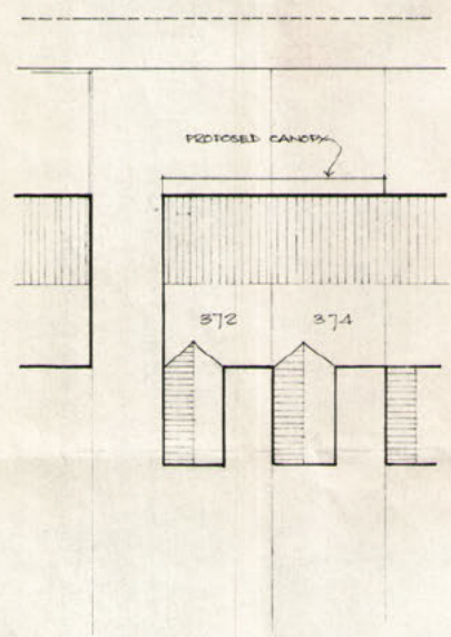
SITE PLAN. scale 1/2" = 1'-0"
