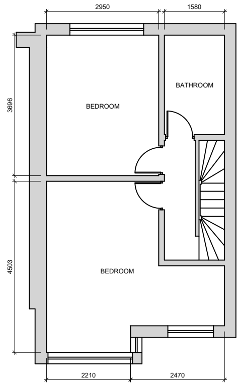
2 EXISTING 1ST FLOOR PLAN SCALE: 1:100
