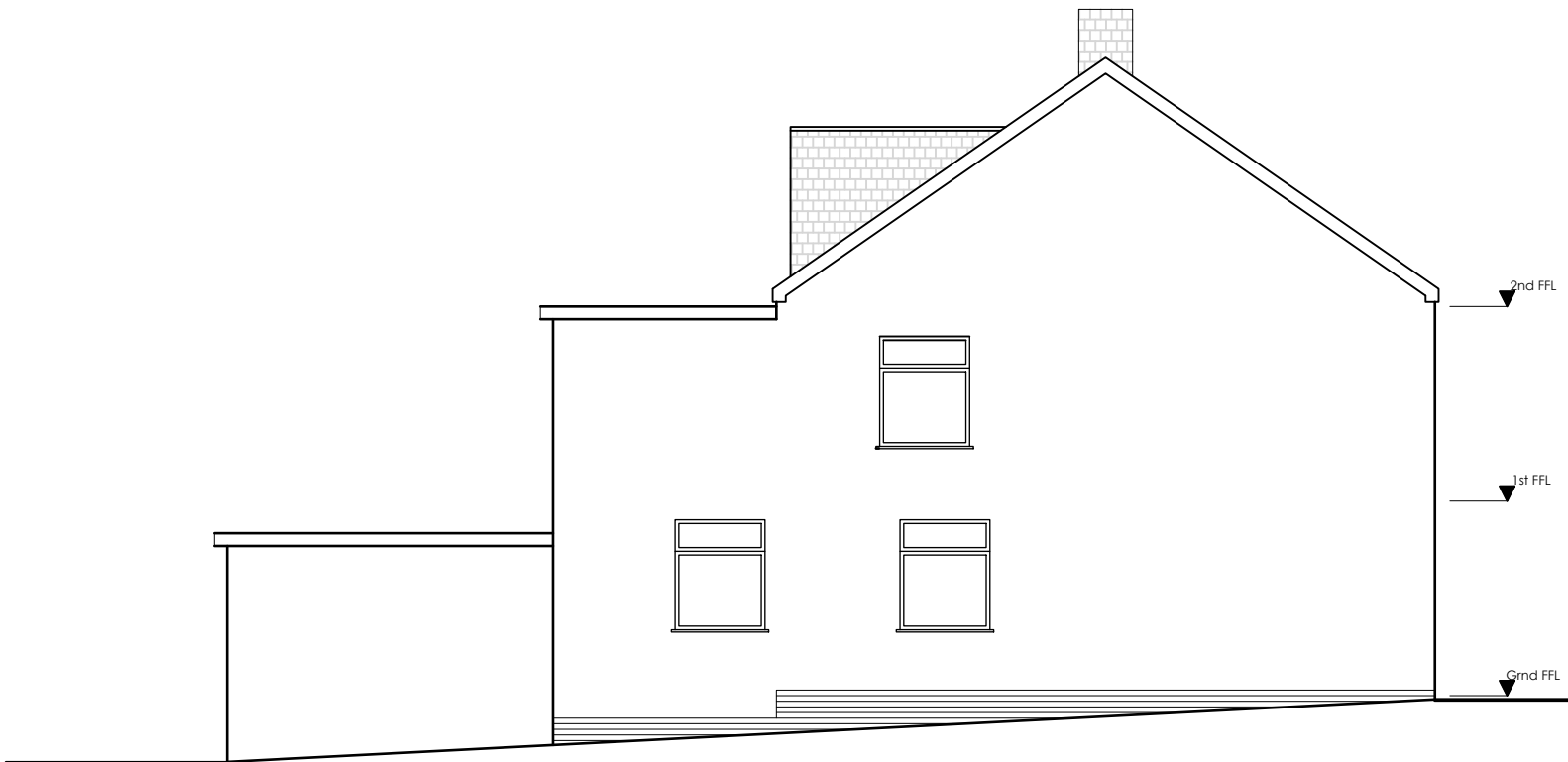
3 PROPOSED SIDE ELEVATION SCALE: 1:100
