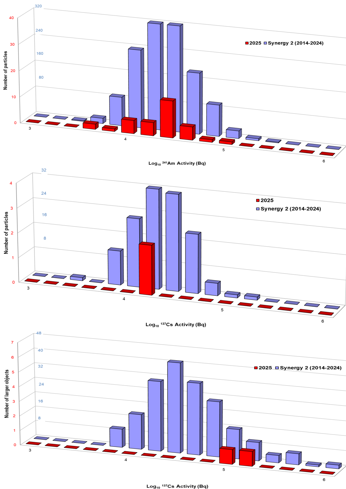
Figure 2: Radioactivity of finds classified as Alpha-rich particles (top), beta-rich particles (middle) and beta-rich larger objects between May 2014 - December 2024 (termed "Synergy2" and shown in blue) compared to data from 2025 (termed "2025" and shown in red).
