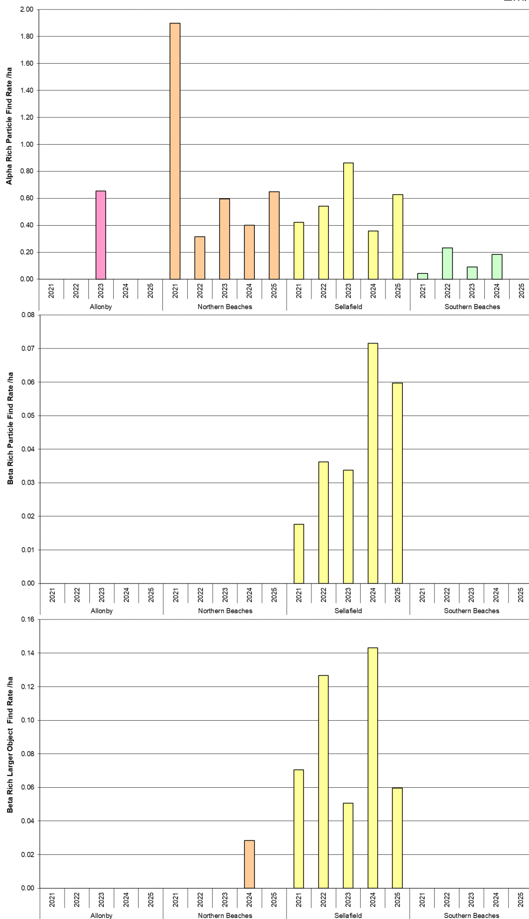
Figure 1: Find rates of Alpha-rich particles (upper), Beta-rich particles (middle) and Beta-rich larger objects (lower) between 2021 - 2024. Note that find rates in 2025 are for finds to date (10 th July) and not the annual rate.
