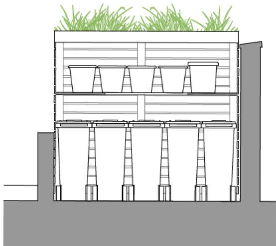
Proposed Bin Store Section at A
