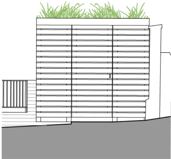
Proposed Bin Store North Elevation
