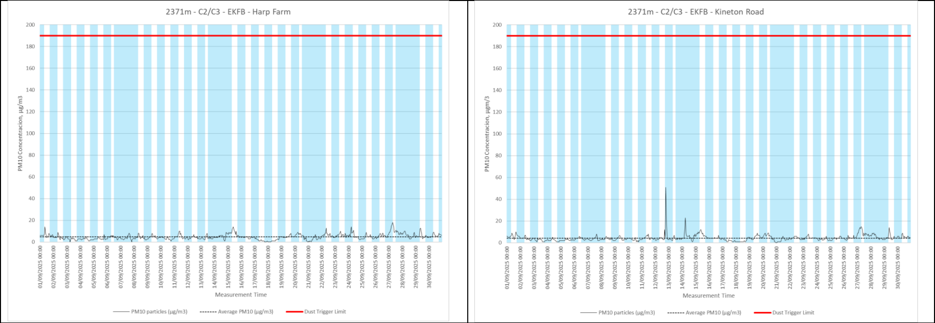
Air Quality and Dust Monitoring Summary Report, September 2025 Stratford-on-Avon District Council Figure 2: Construction dust 1-hour mean indicative PM 10 concentration for all dust monitors
