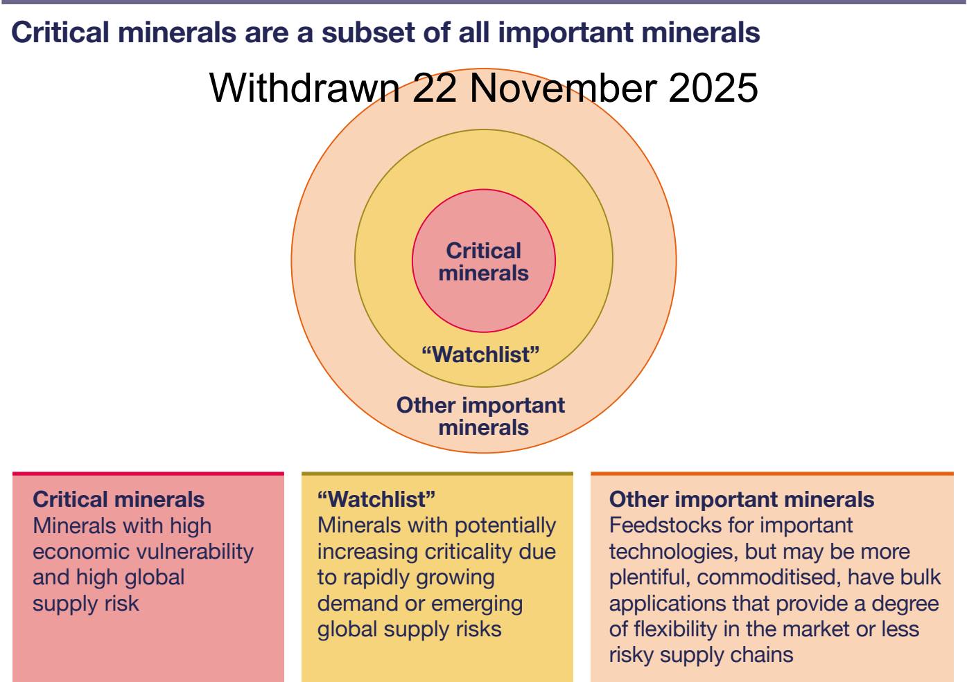
Figure 1: Schematic of critical minerals, as a subset of all important minerals.
