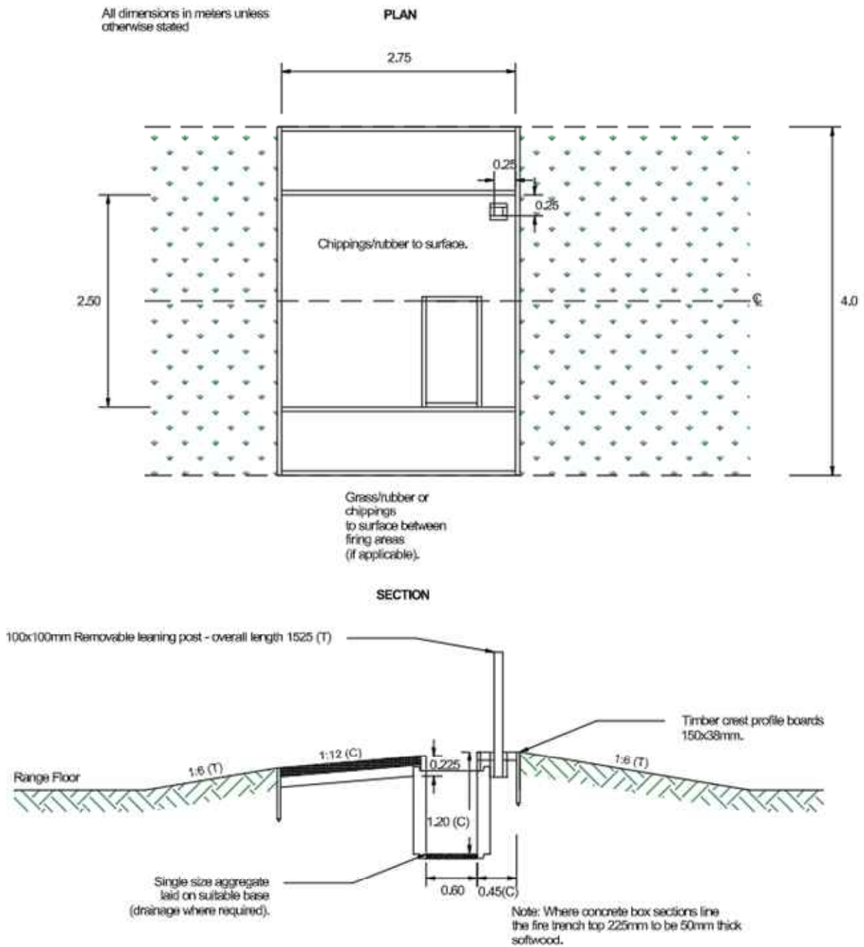
Fig 2 - 16. Standard Firing Point Detail
