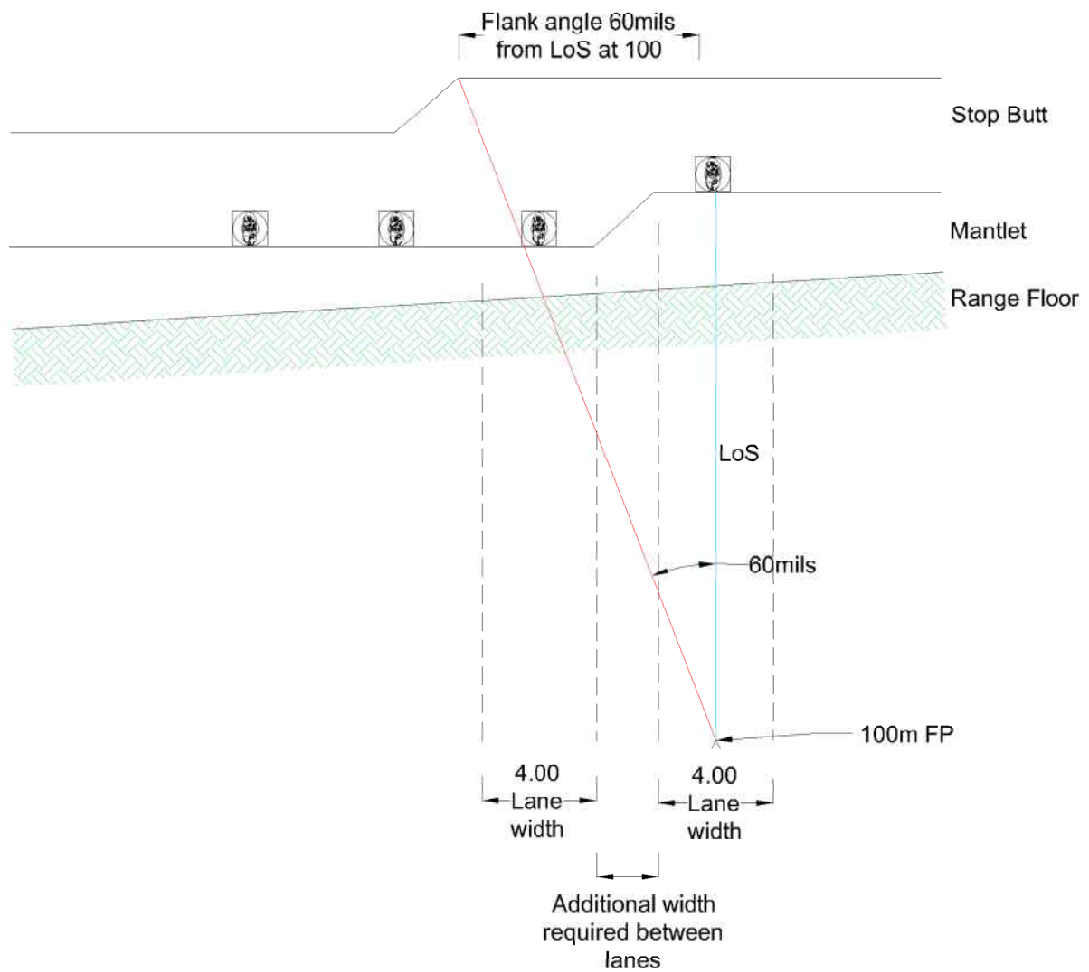
Fig 11 - 5. Stepped Mantlet and Stop Butt
