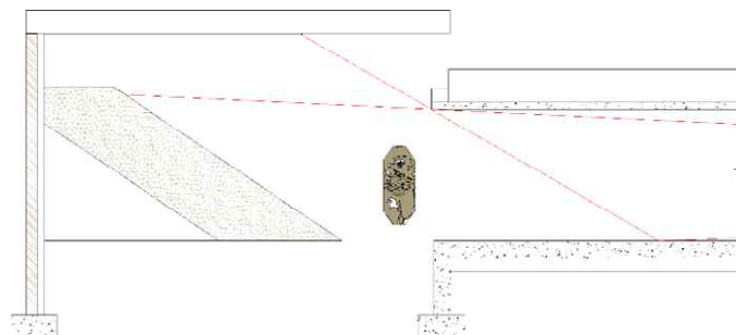
Fig 8 - 2 – Typical Bullet Trap Using Sand Natural Angle of Repose (30° – 34°).
