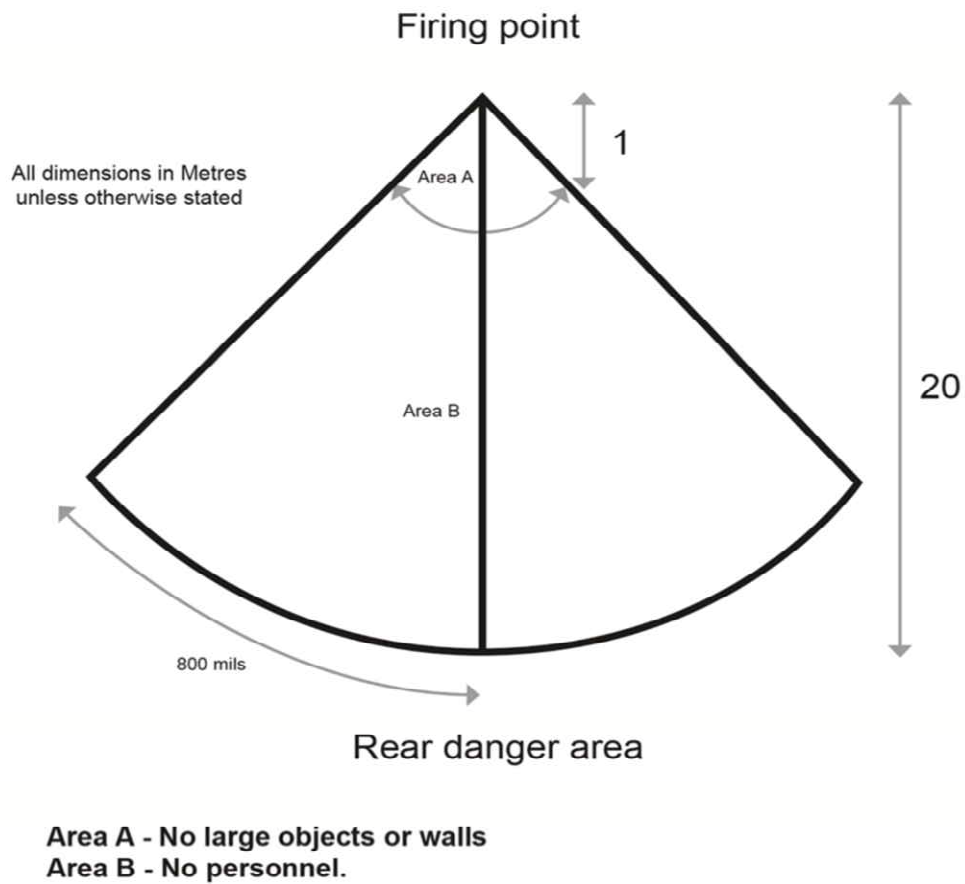
Fig 20 - 2. Rear Danger Area NLAW
