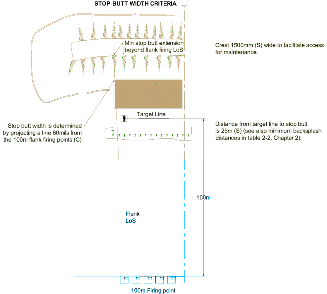
Fig 11 - 3. Determination of Stop Butt Height & Length
