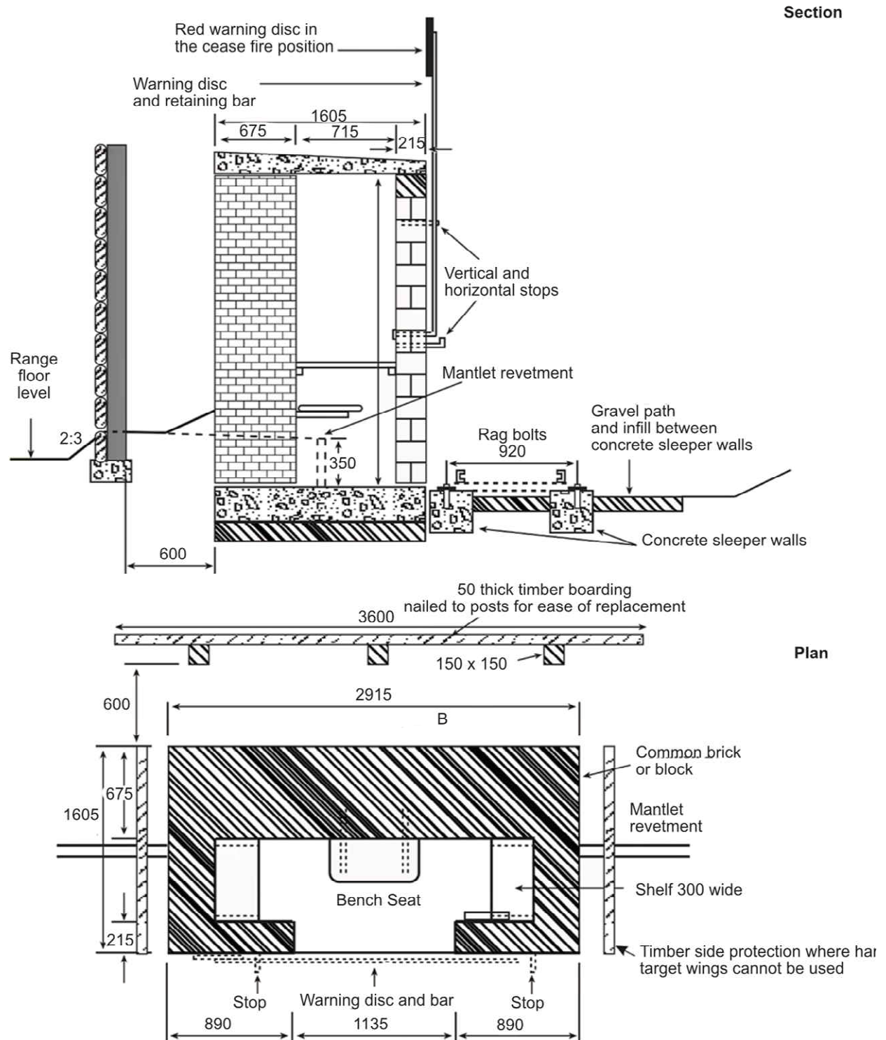
Fig 16 - 4. Markers' Bunker Detail
