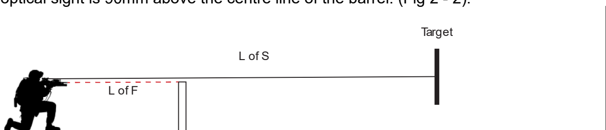
Fig 2 - 2. Line of Fire / Line of Sight
