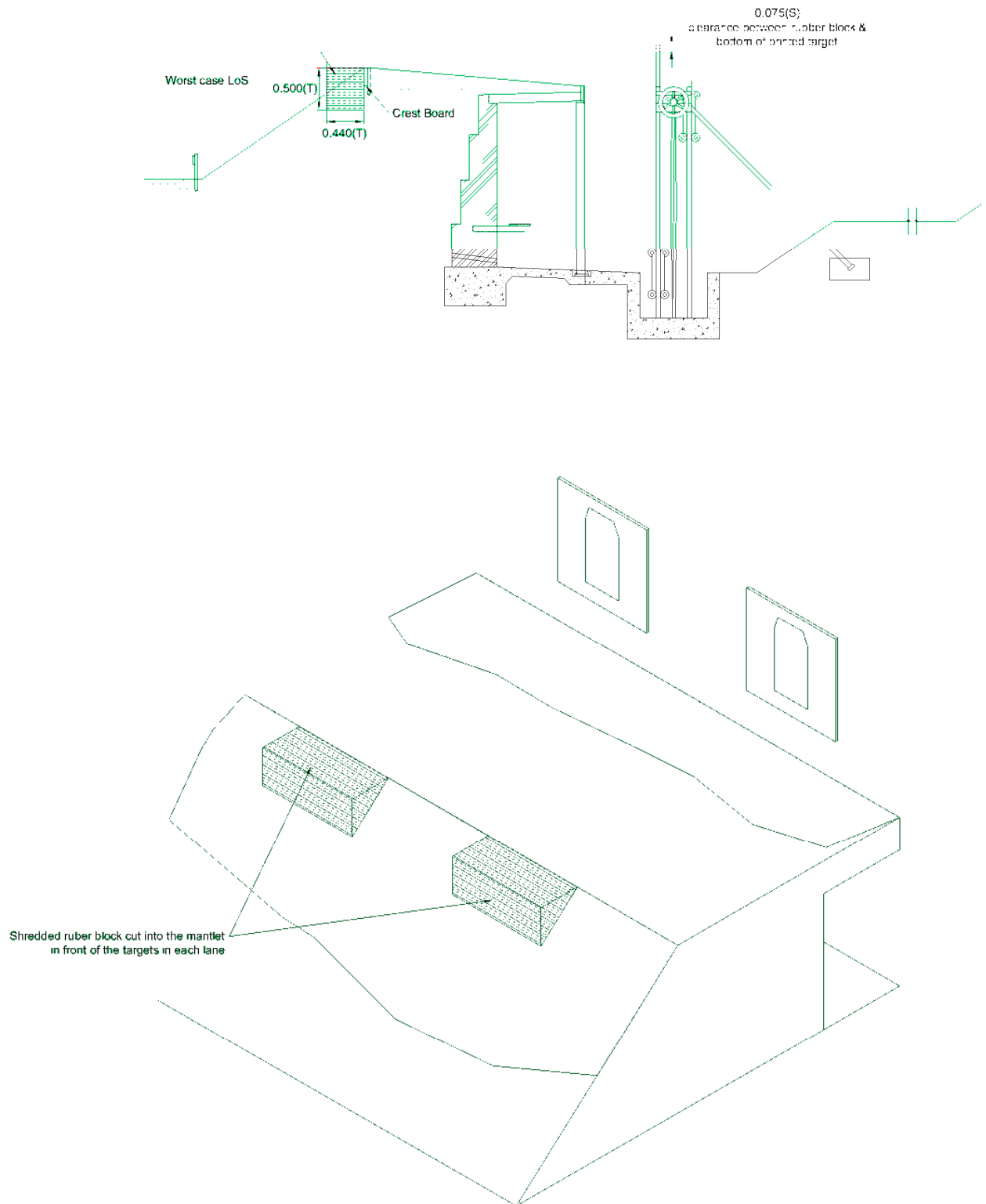
Fig 11 - 12. Mantlet Protection Options for Ease of Maintenance
