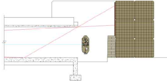
Fig 8 - 1 - Typical Bullet Trap Arrangement.
