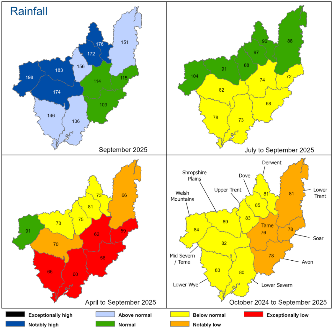
Figure 2.1: Rainfall as % LTA for hydrological areas for the current month (up to 30 September 2025), the last 3 months, the last 6 months, and the last 12 months, relative to an analysis of respective historic totals from 1991 to 2020. Table available in the appendices with detailed information.
