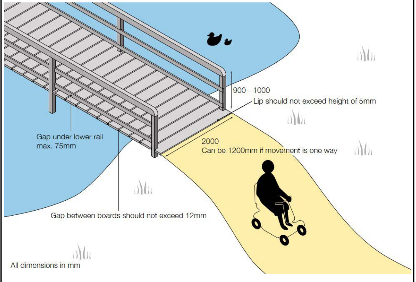
Figure 20: Rural bridge
