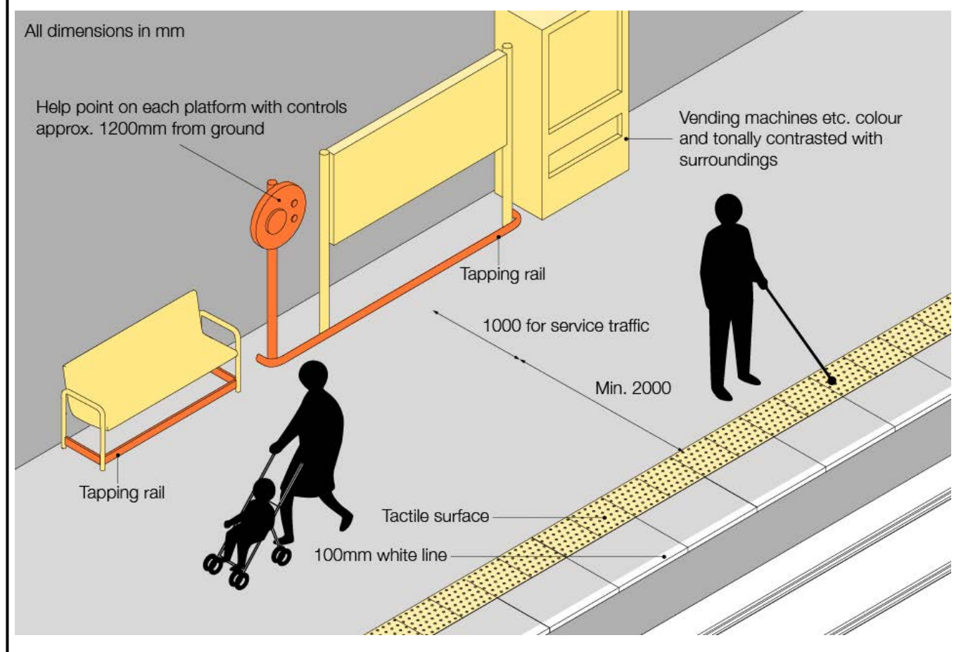
Figure 8: Rail platform
