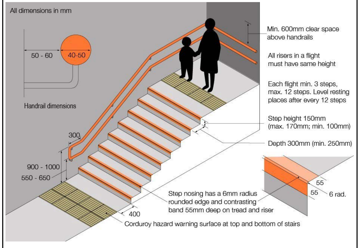
Figure 4: Stairs
