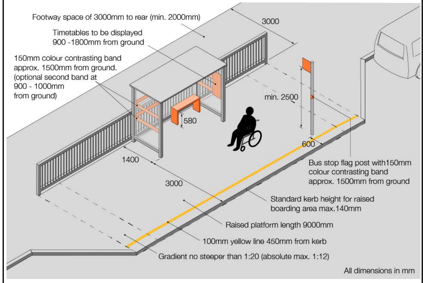
Figure 13: Bus stop
