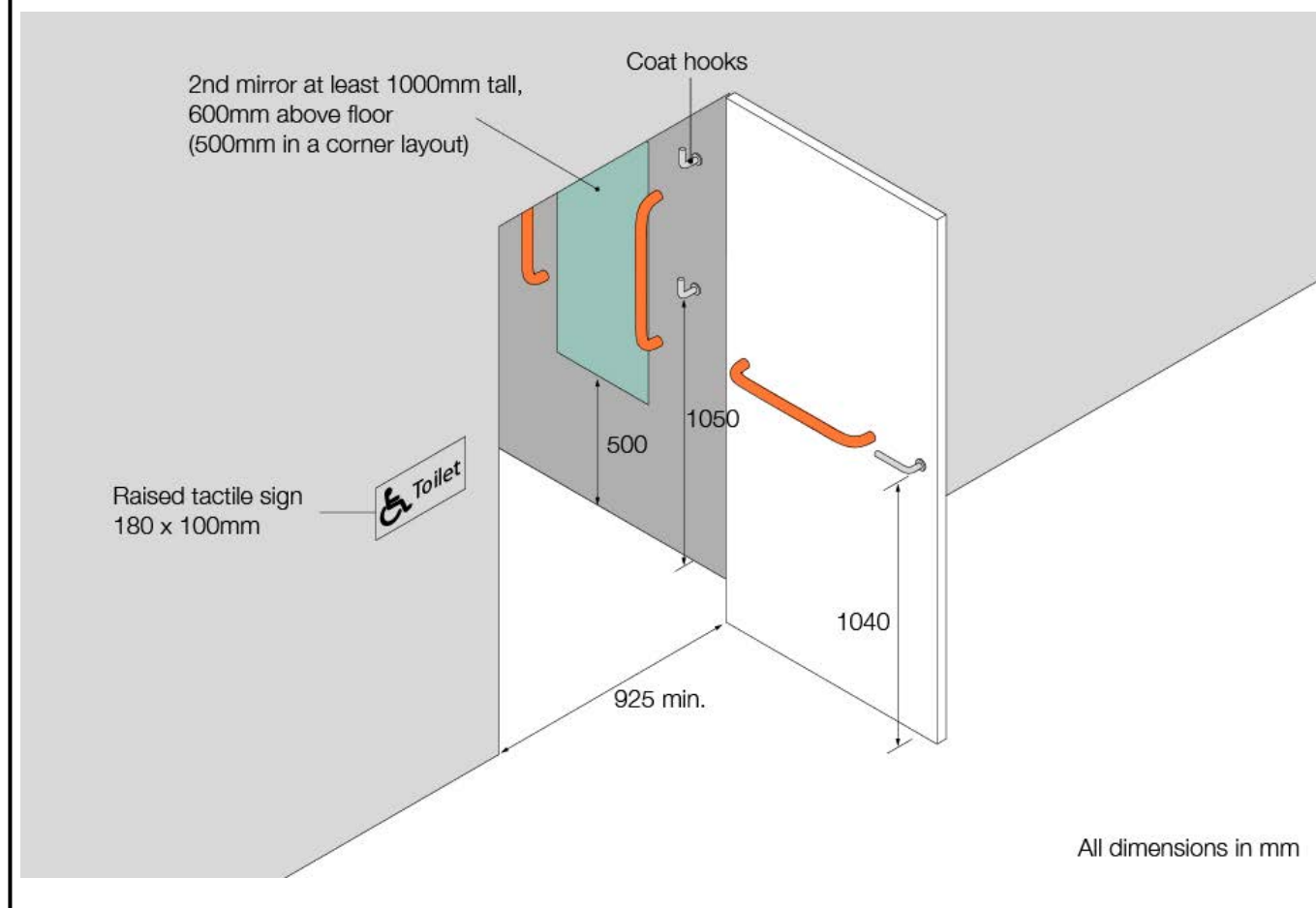
Figure 18: Toilet door
