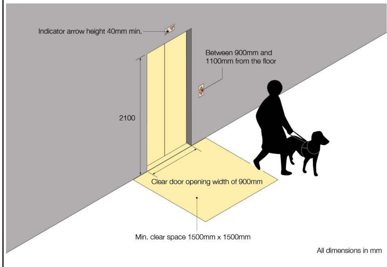
Figure 7: Lift exterior
