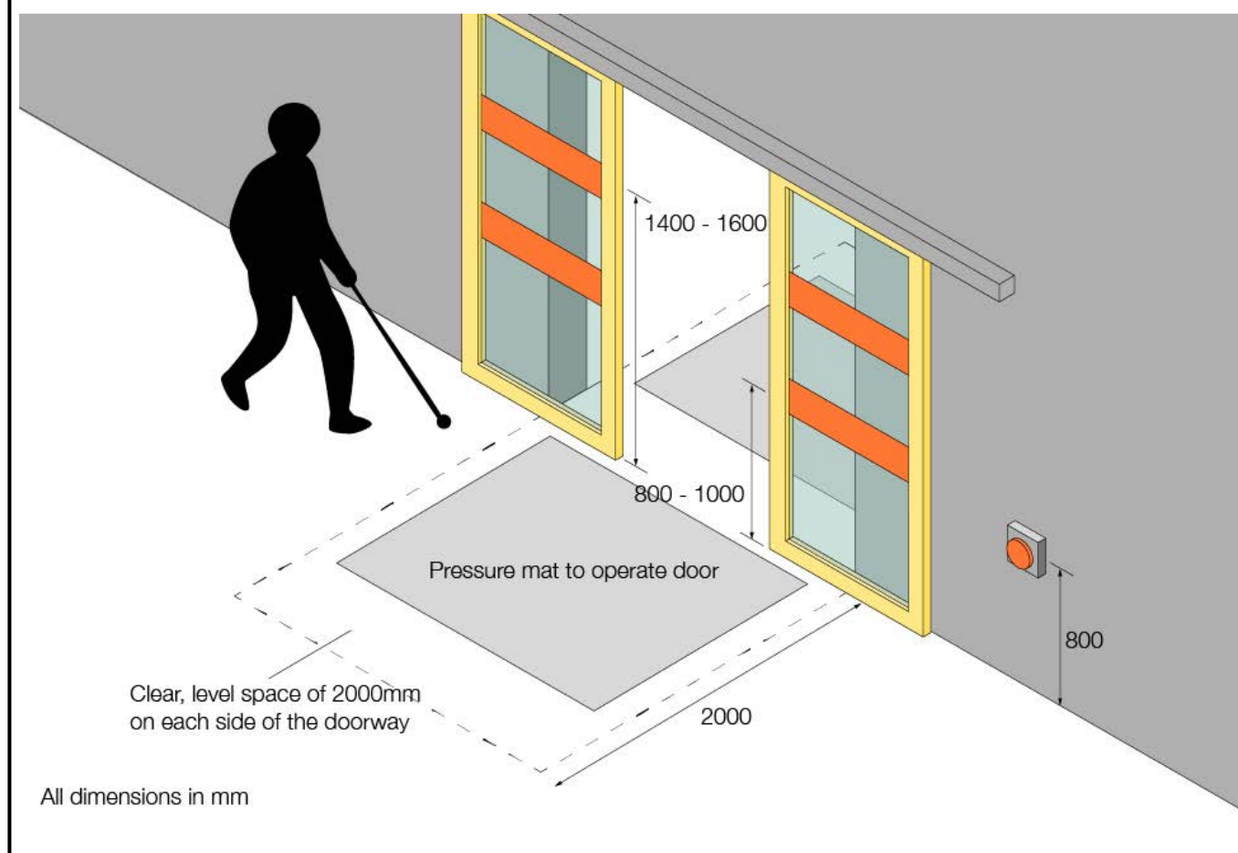
Figure 15: Automatic sliding doors
