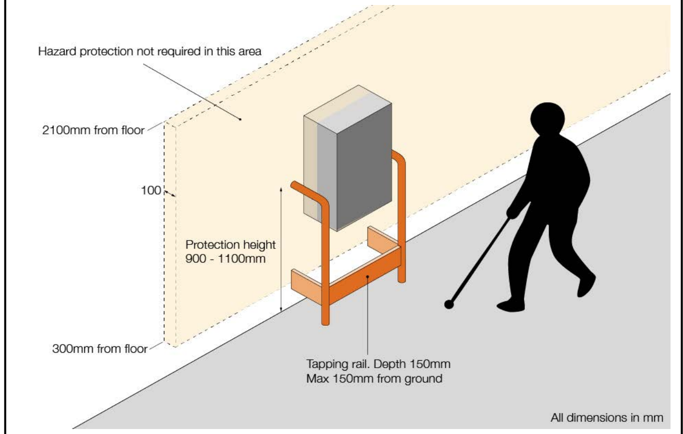
Figure 2: Low-level obstructions
