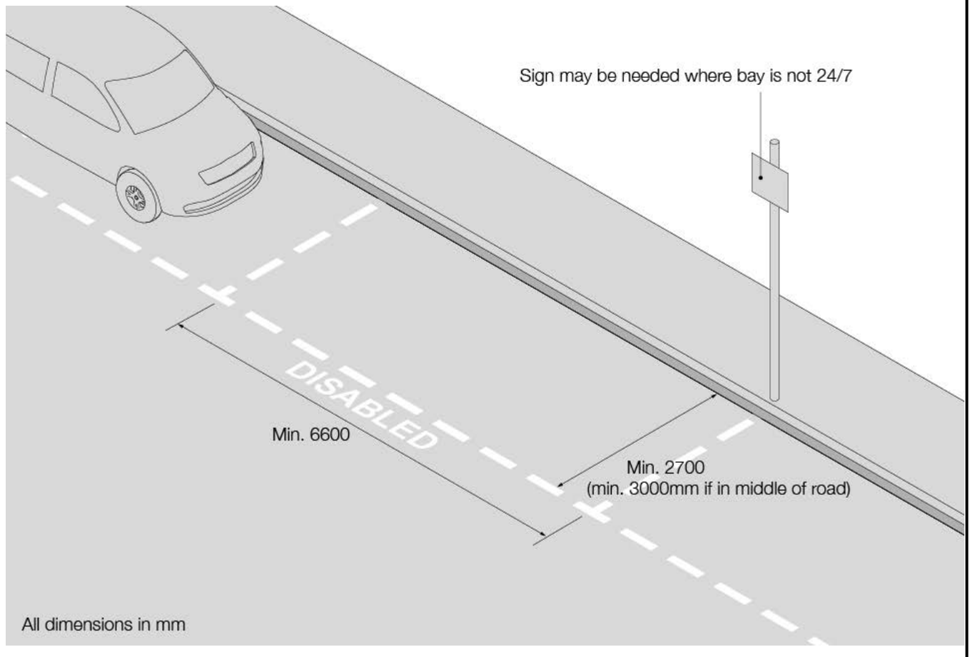
Figure 12: On-street parking parallel to a kerb
