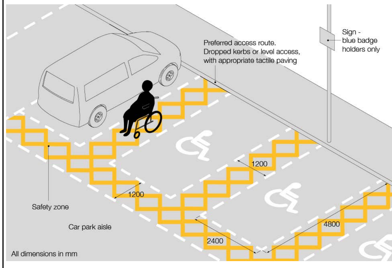
Figure 10: Off-street parking
