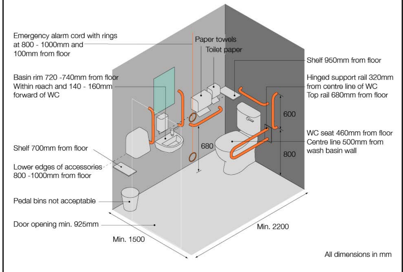
Figure 19: Toilet interior
