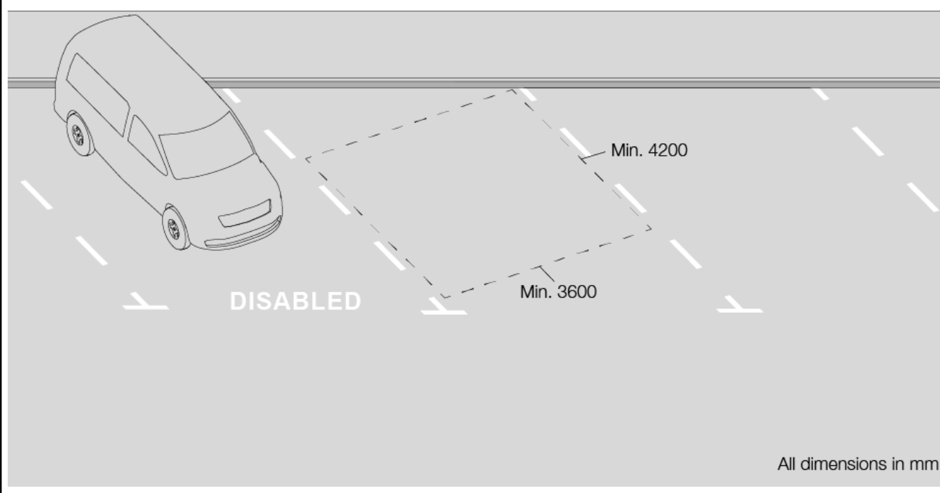
Figure 11: On-street parking at an angle to a kerb
