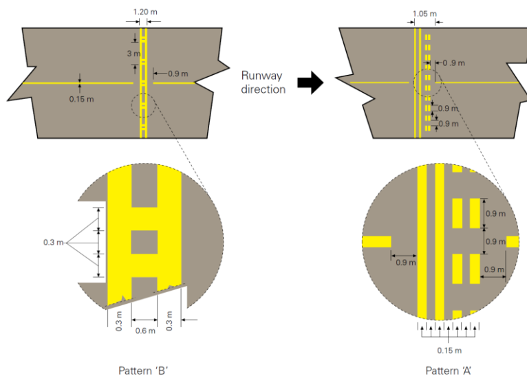
Figure 6. Holding Position Patterns
