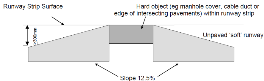
Figure 1. Delethalization
