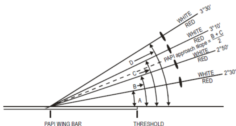
Figure 1. Light beams and angle of elevation setting of PAPI and Abbreviated PAPI
