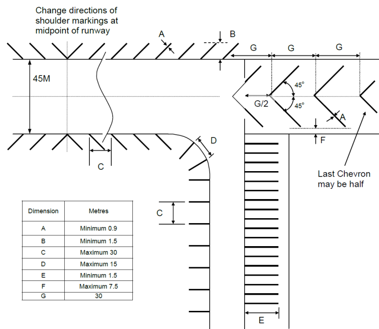
Figure 5. – Hazardous Area Markings
