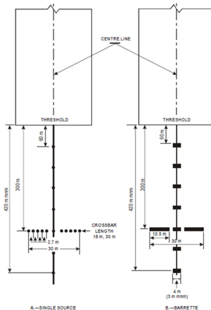
▶ Figure 1. Simple Approach Lighting System. ◀
