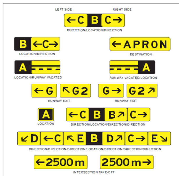
Figure 2. Airfield Sign Layout
