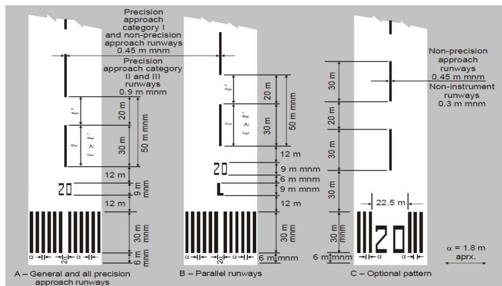
Figure 3. Runway designation, centre-line and threshold markings
