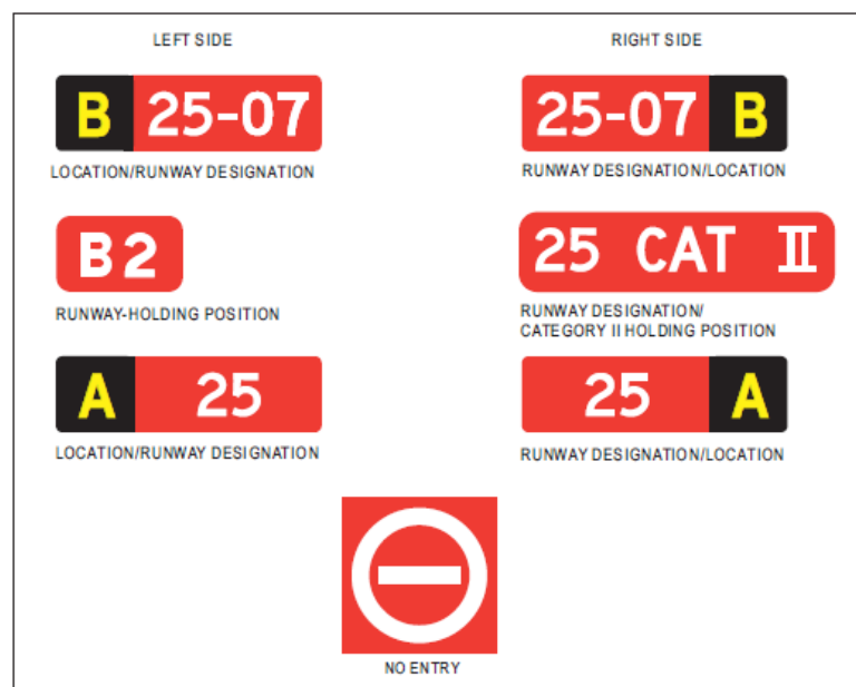
Figure 1. Intermediate holding signs
