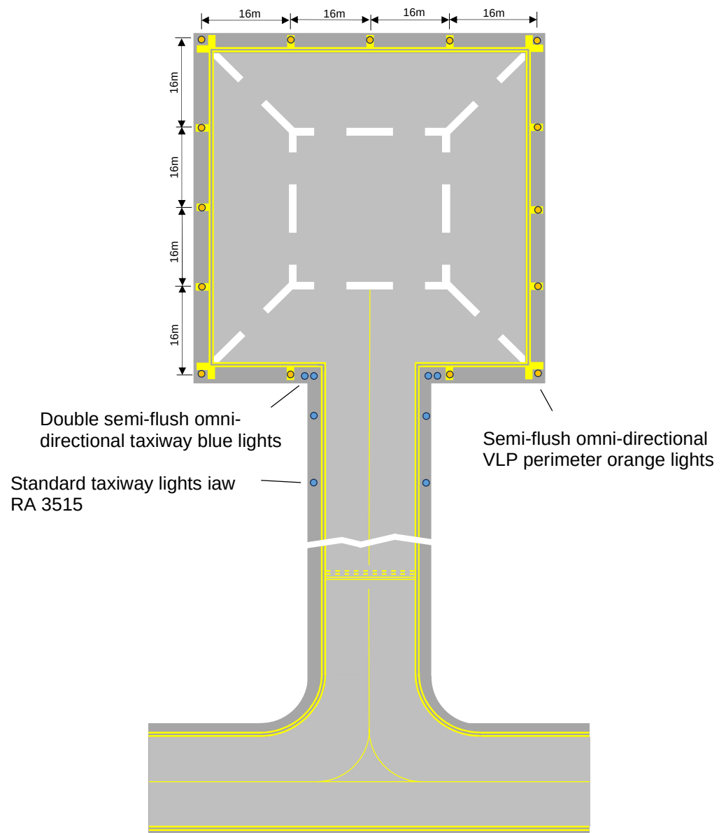
Figure 5 – VLP AGL Layout
