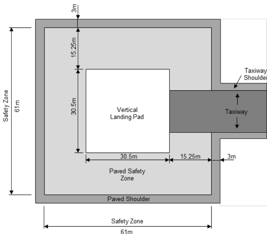
Figure 1 – Vertical Landing Pad Dimensions.
