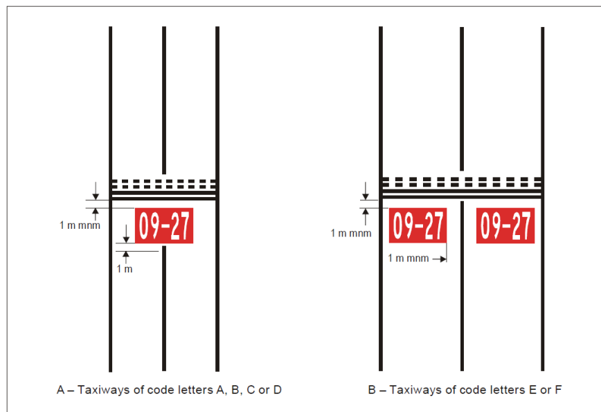
Figure 14. Mandatory Instruction Markings
