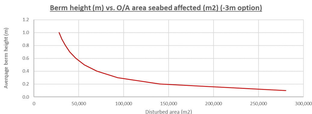
Figure 2.3.5: Mooring line recovery berm height vs. O/A area affected (-3 m option)
