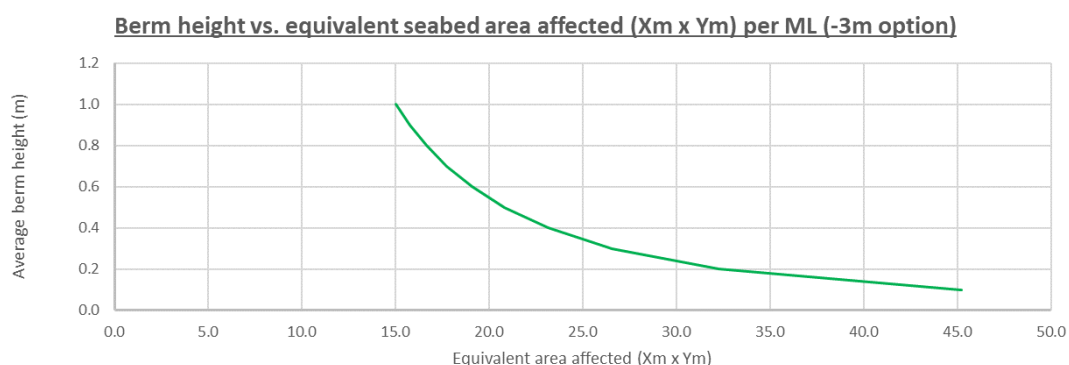
Figure 2.3.6: Mooring line recovery berm height vs. area affected per ML (-3 m option)
