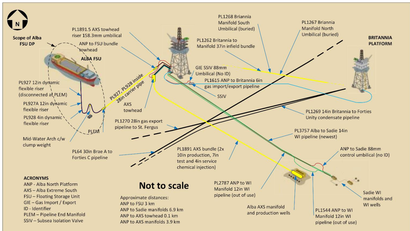
Figure 2.1.2: Alba field installations and infrastructure (not to scale)
