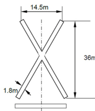
Runway C/L
