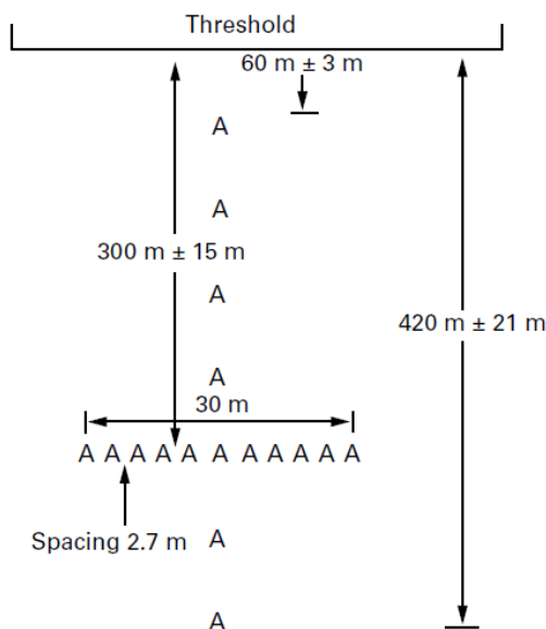
Figure 1. Simple Approach Lighting System.
