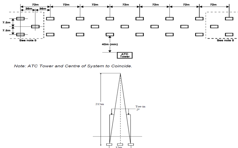
Figure 8. Undercarriage Inspection System Lights
