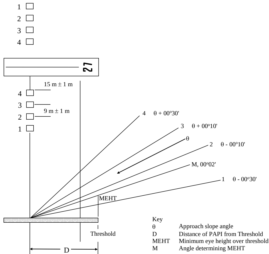
Figure 4. Approach Slope Definition
