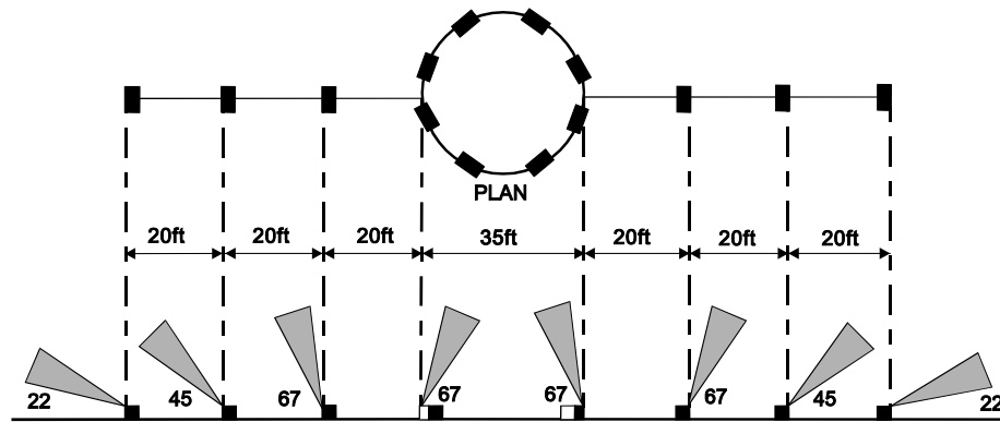
Undercarriage Check Flarepath – Layout and Optical Requirements
