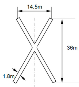
Runway C/L
