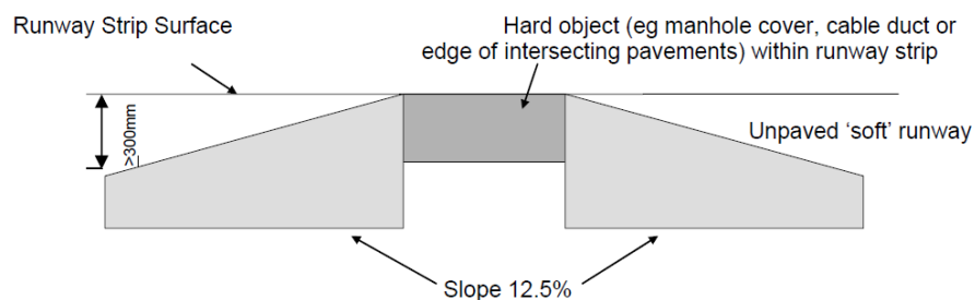
Figure 1. De-lethalization
