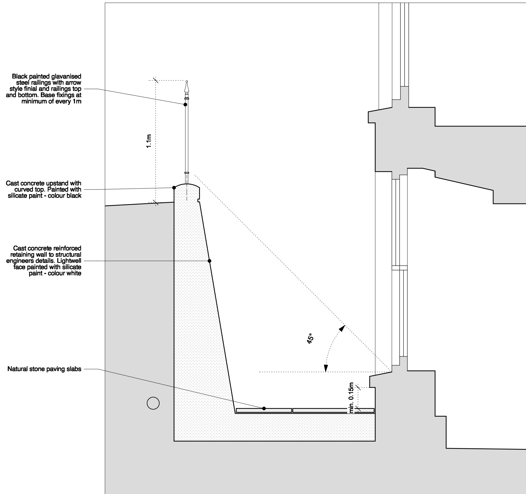
Front Lightwell Section
