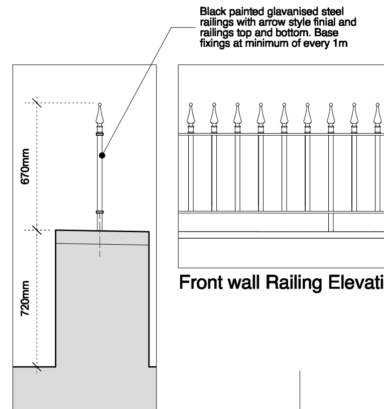
Front Wall Railing Section
