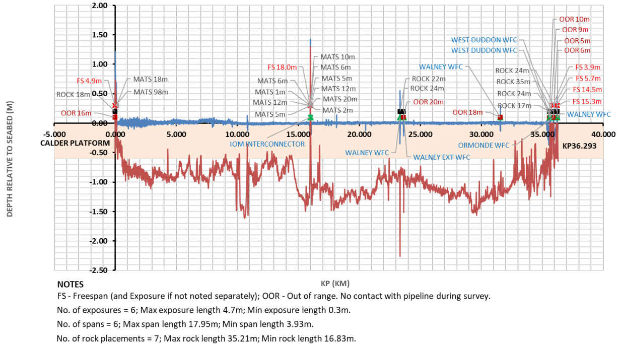
Figure 3.4.7: PL1965 & PL1966 burial profile (2022)
