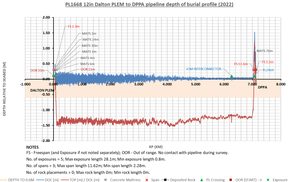
Figure 3.5.3: PL1668 pipeline burial profile (2022)
