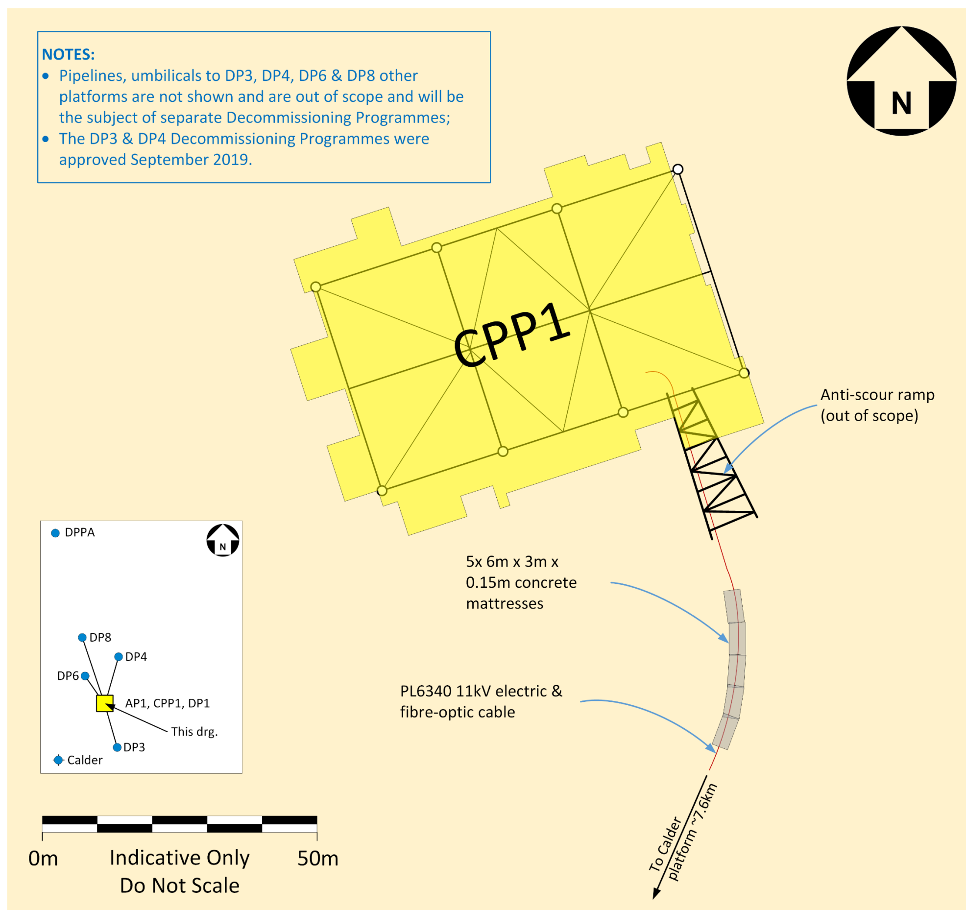
Figure B.7.1: South Morecambe CPP1 approach schematic (PL6340)
