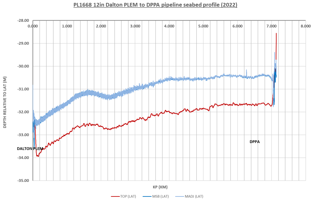
Figure 3.5.2: PL1668 pipeline seabed & burial profile (2022)
