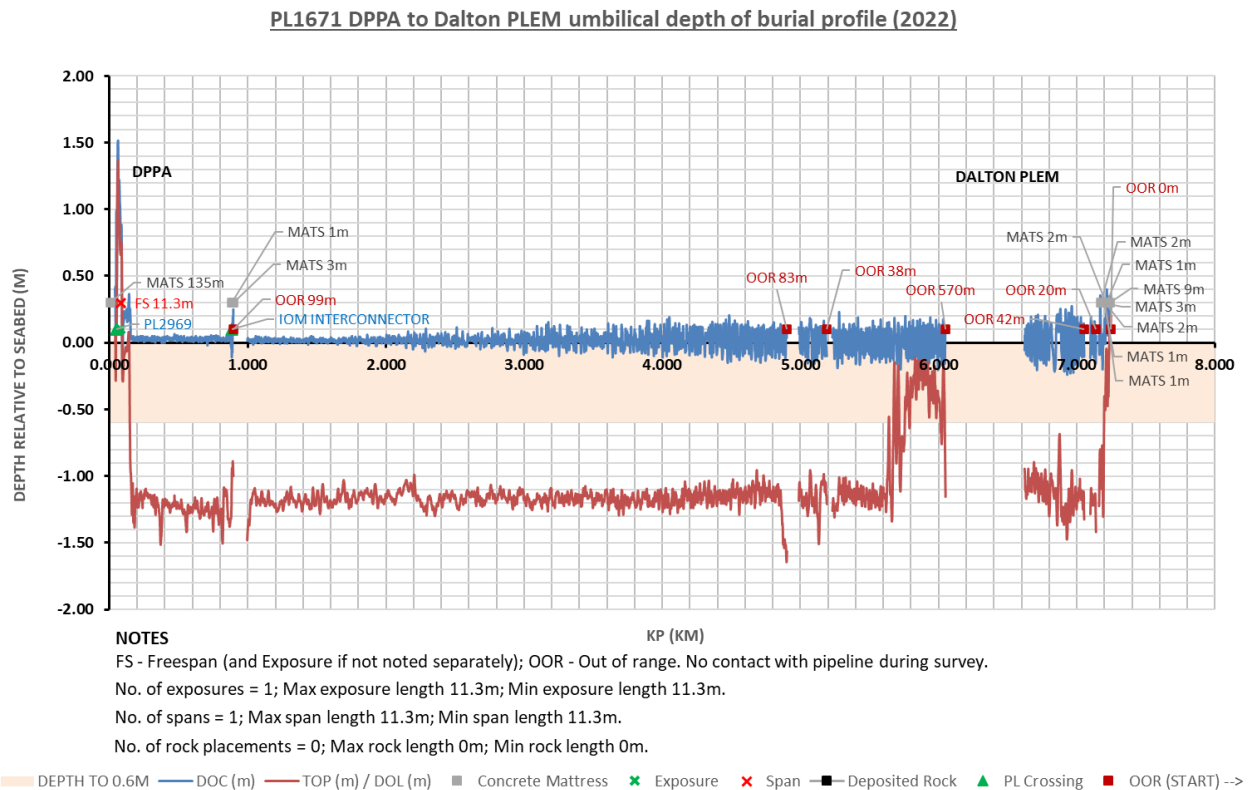
Figure 3.5.9: PL1671 umbilical burial profile (2022)
