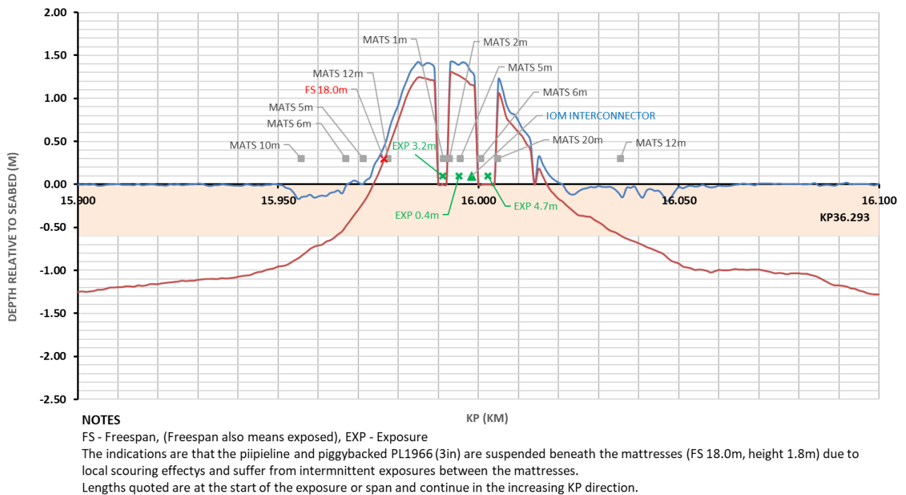
Figure 3.4.8: PL1965 & PL1966 burial profile between KP15.9-KP16.1 (2022)
