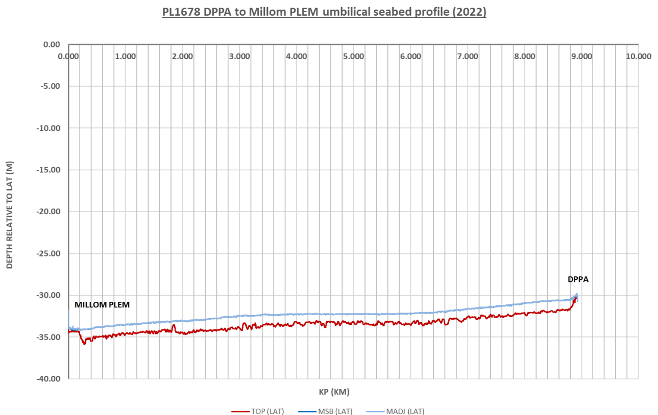
Figure 3.6.10: PL1678 umbilical seabed & burial profile (2022)
