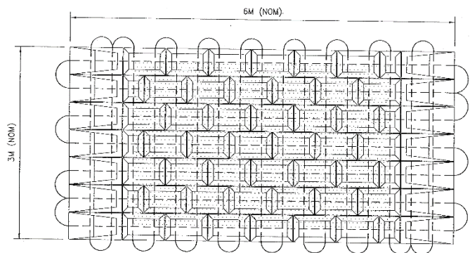
Figure 2.4.18: Typical concrete and concrete fronded mattresses (6m x 3m x 0.15m)
