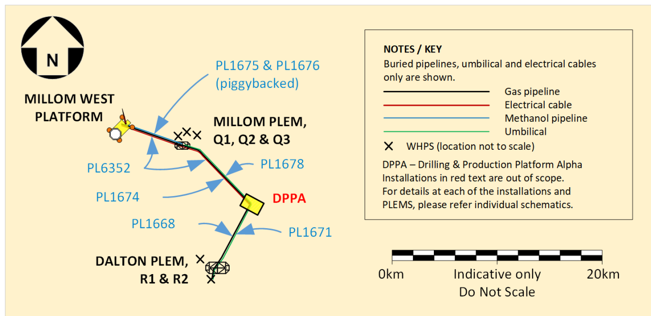
Figure 2.2.3: Layout of Dalton & Millom in relation to each other
