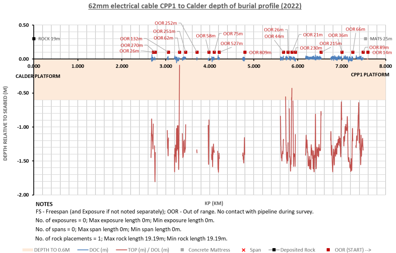
Figure 3.4.16: PL6340 electrical cable from CPP1 to Calder burial profile (2022)
