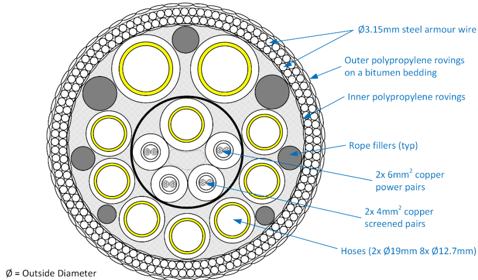
DPPA to Dalton & Millom PLEM Umbilical (Ø113mm)
