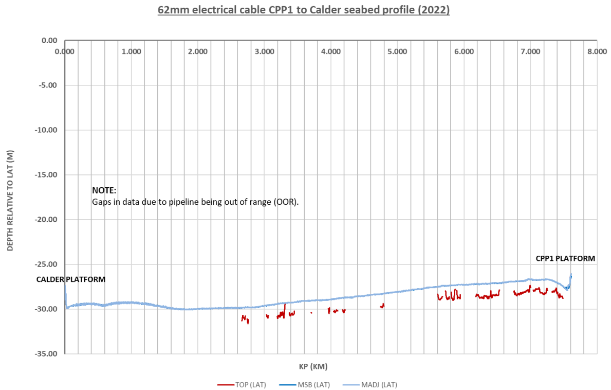
Figure 3.4.15: PL6340 electrical cable from CPP1 to Calder seabed & burial profile (2022)
