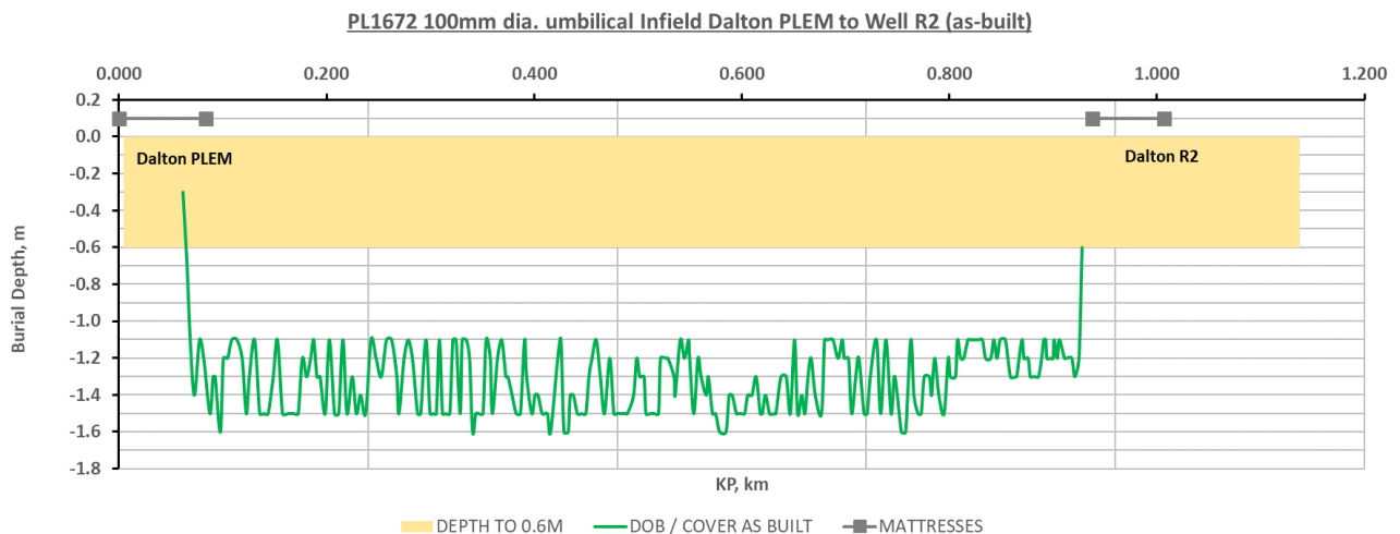
Figure 3.5.10: PL1672 umbilical 'as-built' burial profile
