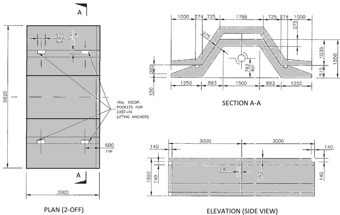
Figure 2.3.1: Millom PLEM Pipeline Protection Units
