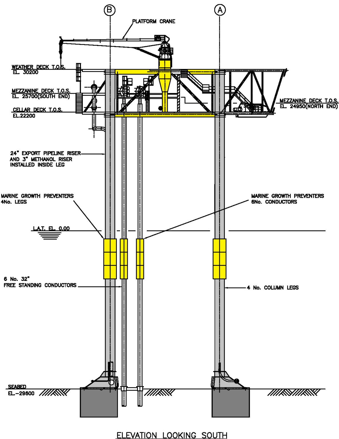
Figure 2.1.3: Calder platform (elevation looking south) 4
