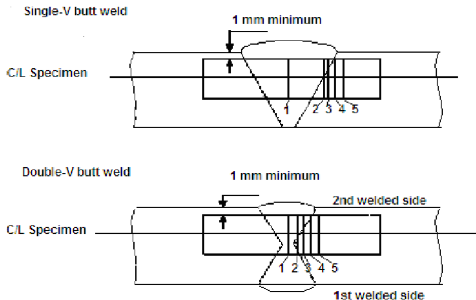
Figure 6.2 – Orientation of weld test specimen
