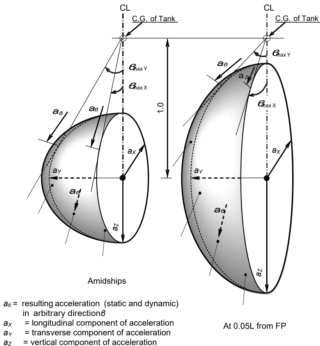
Figure 4.1 – Acceleration ellipsoid
