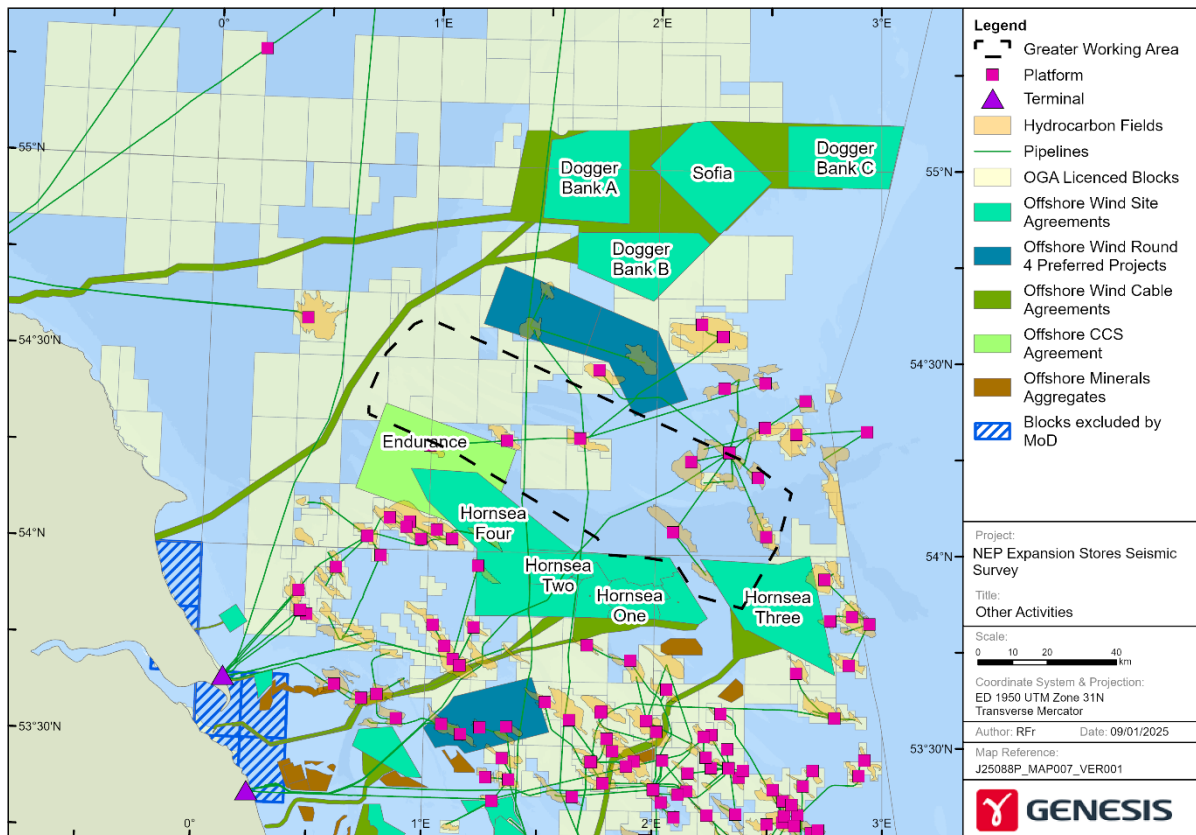
Figure 3: Offshore wind farms and oil and gas activities in the region of the proposed Expansion Store Seismic Survey GWA.
