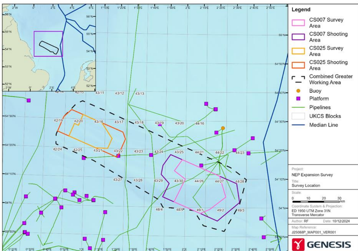
Figure 1: Location of the proposed CS007 Seismic Survey and greater working area.
