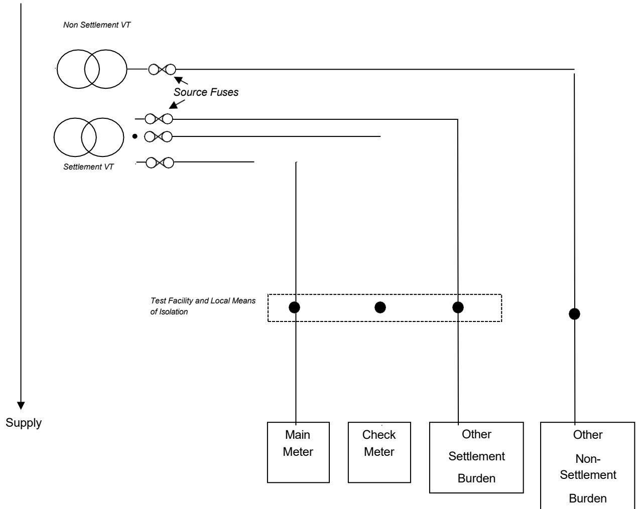
Figure 1: Fusing arrangements for cable runs of more than 30 metres distance between source fusing and local means of isolation 46 47 .
