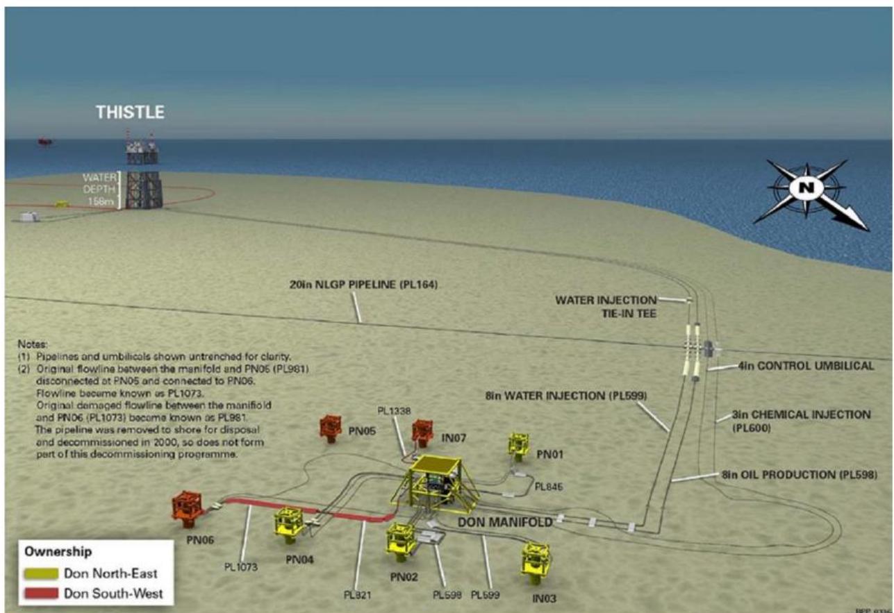
Figure 2.1.1 The Don field assets and infrastructure
