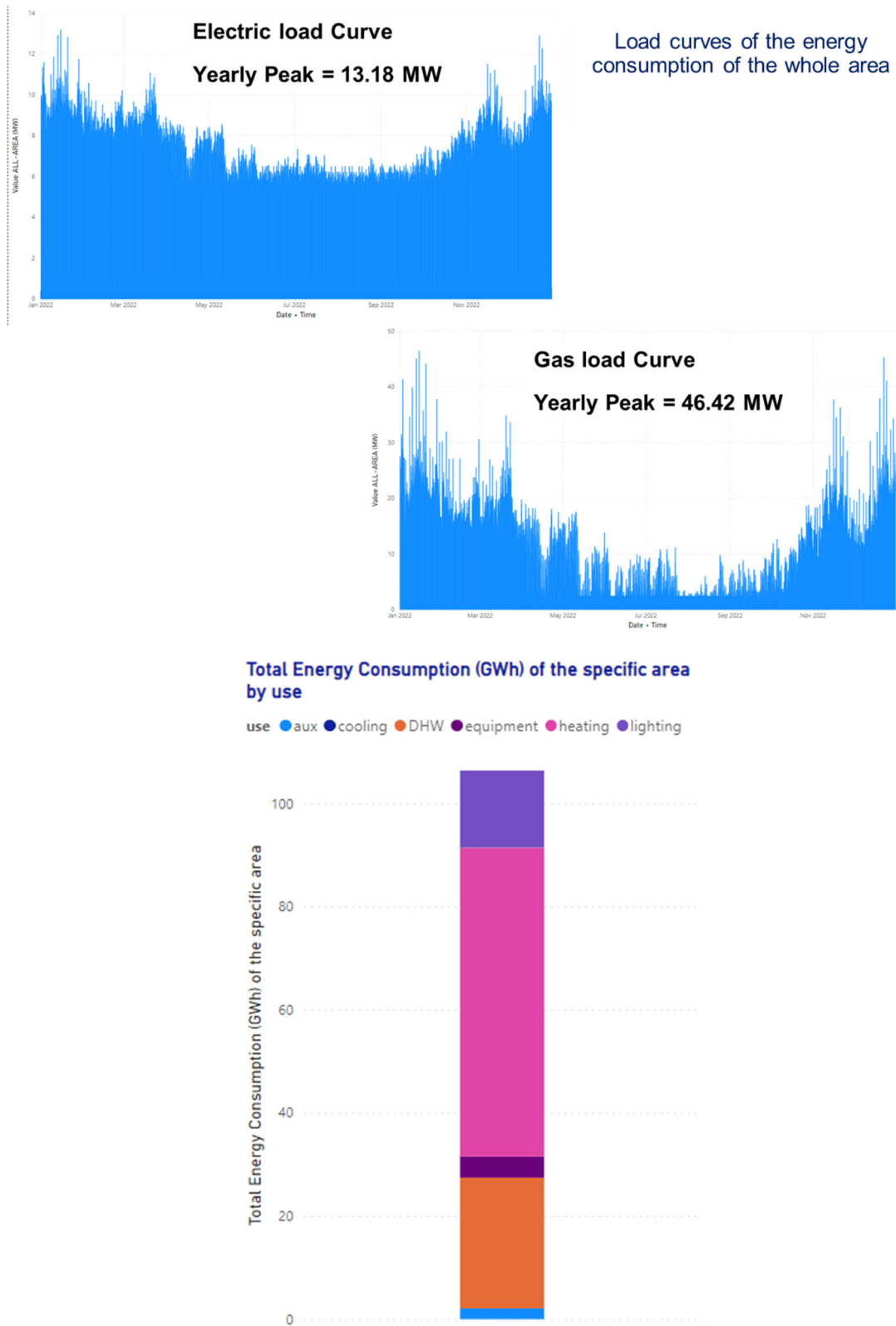
Figure 13: Energy Consumption - Scenario Business as usual
