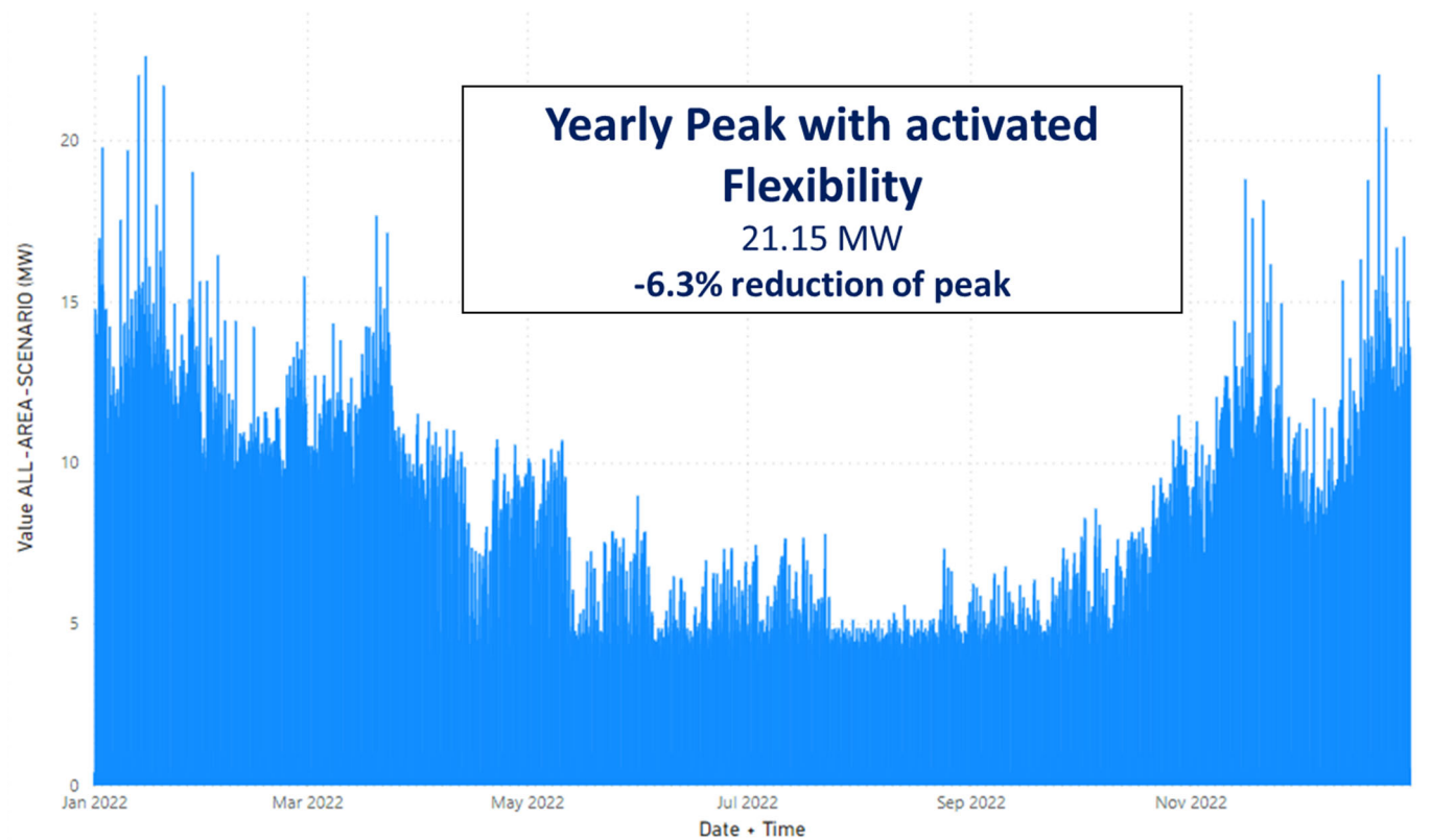
Figure 41: Potential of peak reduction with Flexibility - Scenario Flexibility (with HP scenario)
