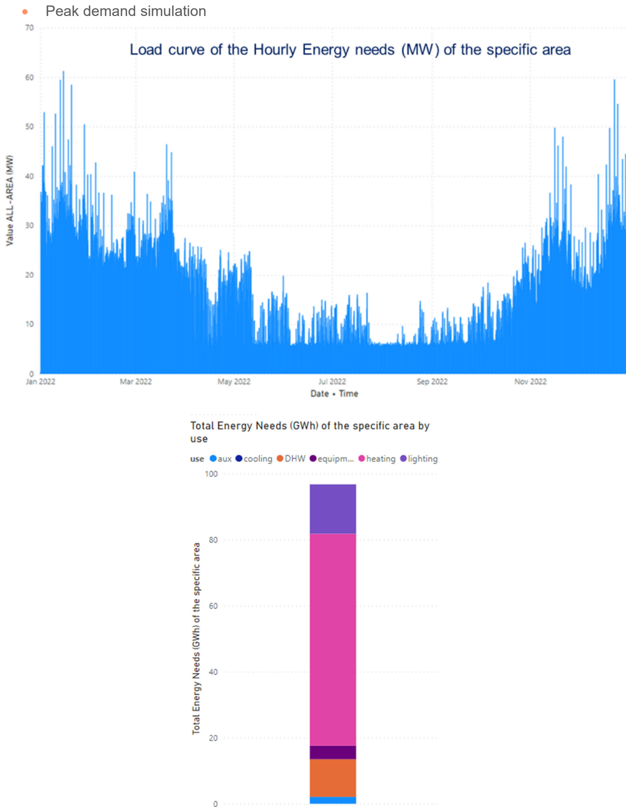
Figure 12: Energy Needs - Scenario Business as usual
