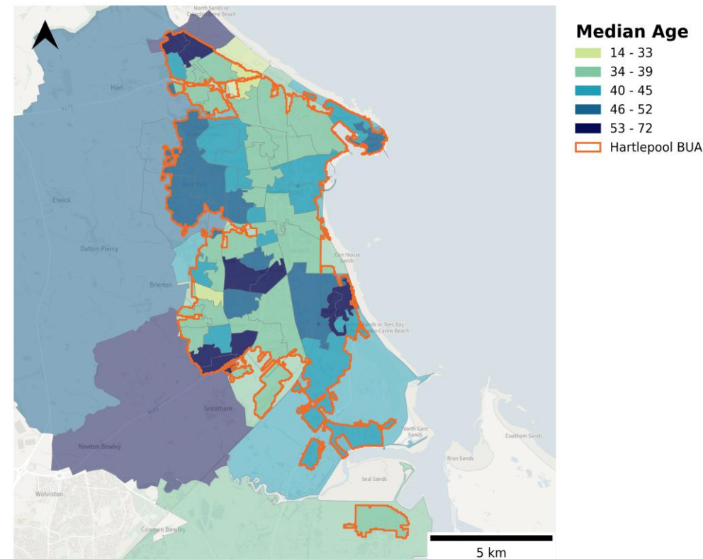
Median age in Hartlepool (BUA) at LSOA level (2022)
