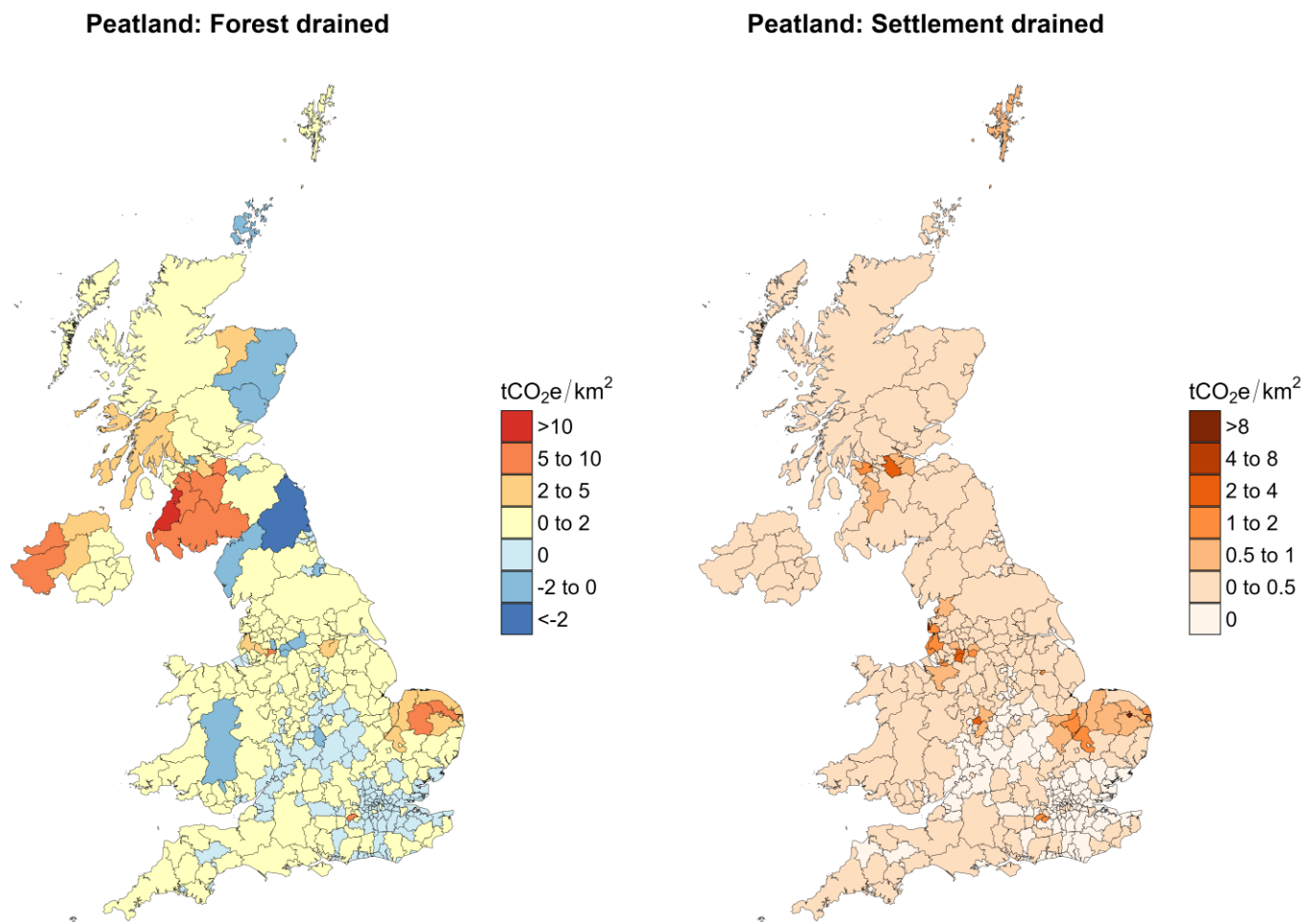
Figure 9: Net carbon dioxide, methane and nitrous oxide emissions from Peatlands: Forest drained and Settlement drained per local authority area (tCO 2 e/km 2 ) in 2023.
