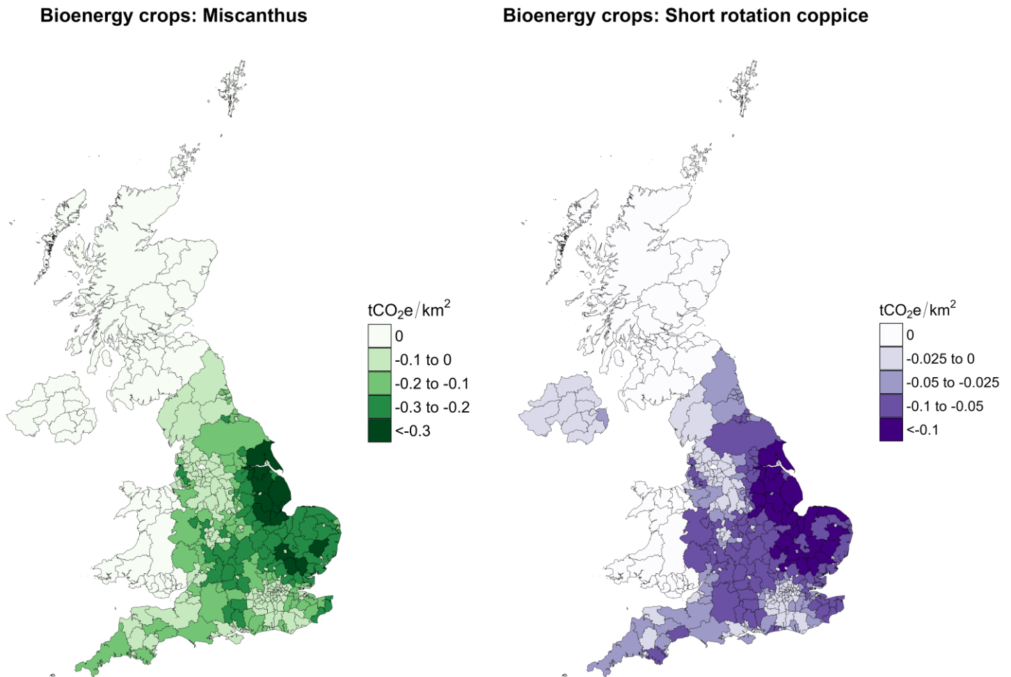
Figure 17: Distribution of Bioenergy crops: Miscanthus and Short rotation coppice net emissions/ removals (tCO 2 e/km 2 ) in 2023.
