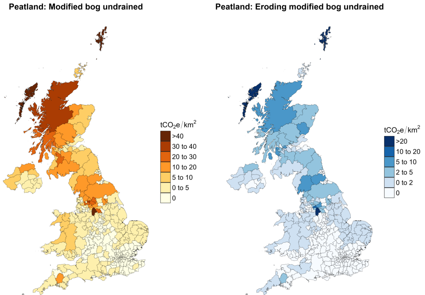
Figure 11: Net carbon dioxide, methane and nitrous oxide emissions from Peatlands: Modified bog undrained and Eroding modified bog undrained per local authority area (tCO 2 e/km 2 ) in 2023.
