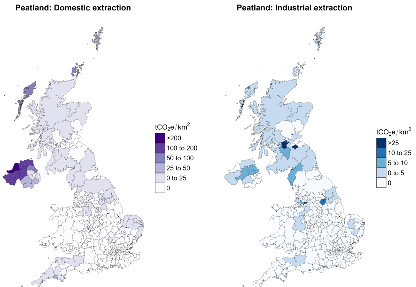
Figure 8: Net carbon dioxide, methane and nitrous oxide emissions from Peatlands: Domestic extraction and Industrial extraction per local authority area (tCO 2 e/km 2 ) in 2023.
