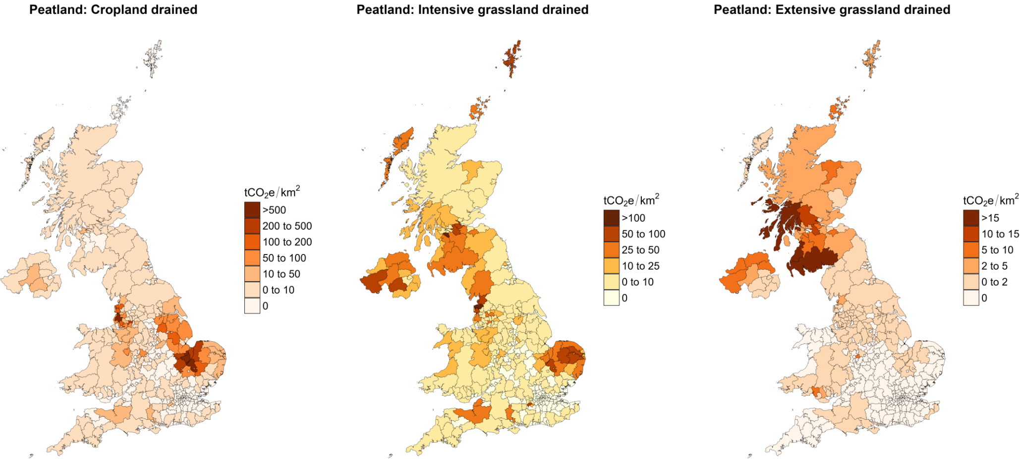
Figure 7: Net carbon dioxide, nitrous oxide and methane emissions Peatland: Cropland drained, Intensive Grassland drained, and Extensive Grassland drained per local authority area (tCO 2 e/km 2 ) in 2023.
