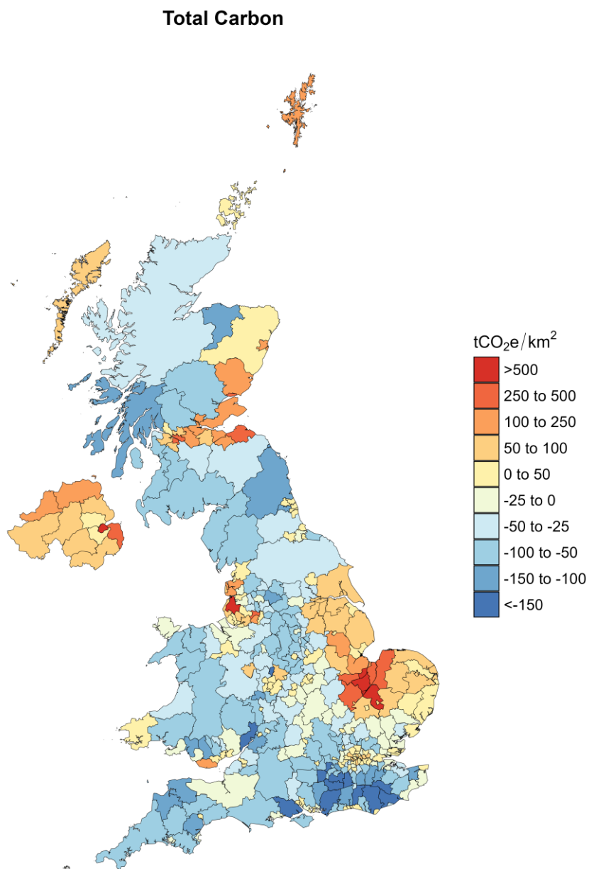
Figure 20: Emissions or removals of carbon from land use, land-use change and forestry per local authority area (tCO 2 e/km 2 ) in 2023.
