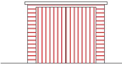
FRONT ELEVATION (EAST)
