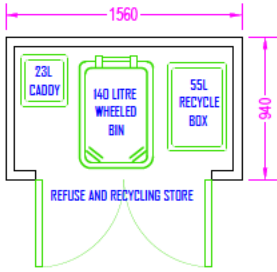
PROPOSED REFUSE AND RECYCLE STORE PLAN 1:50 @ A3
