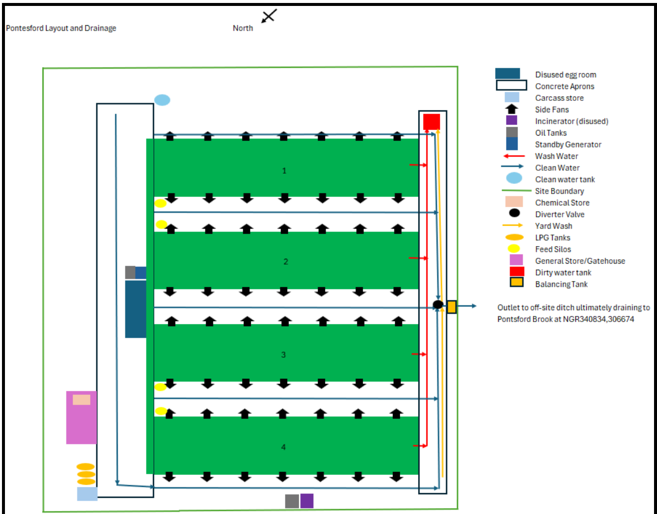
Site layout plan
