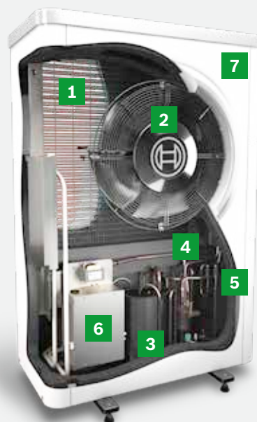
Outdoor unit air to water heat pump
