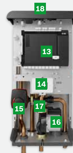
Hybrid indoor unit
