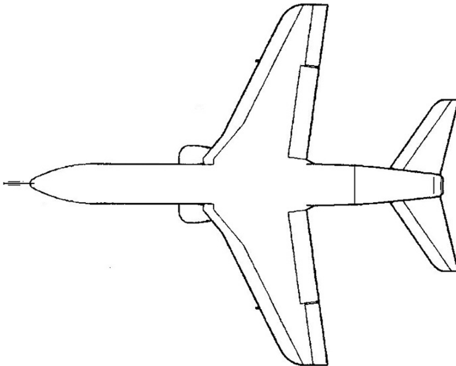
Hawk TMk1/1A Physical Damage Review Map - Lower Surface View
